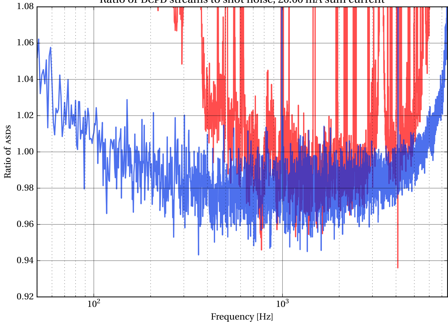
Ratio of DCPD streams to shot noise, 20.00 mA sum current
