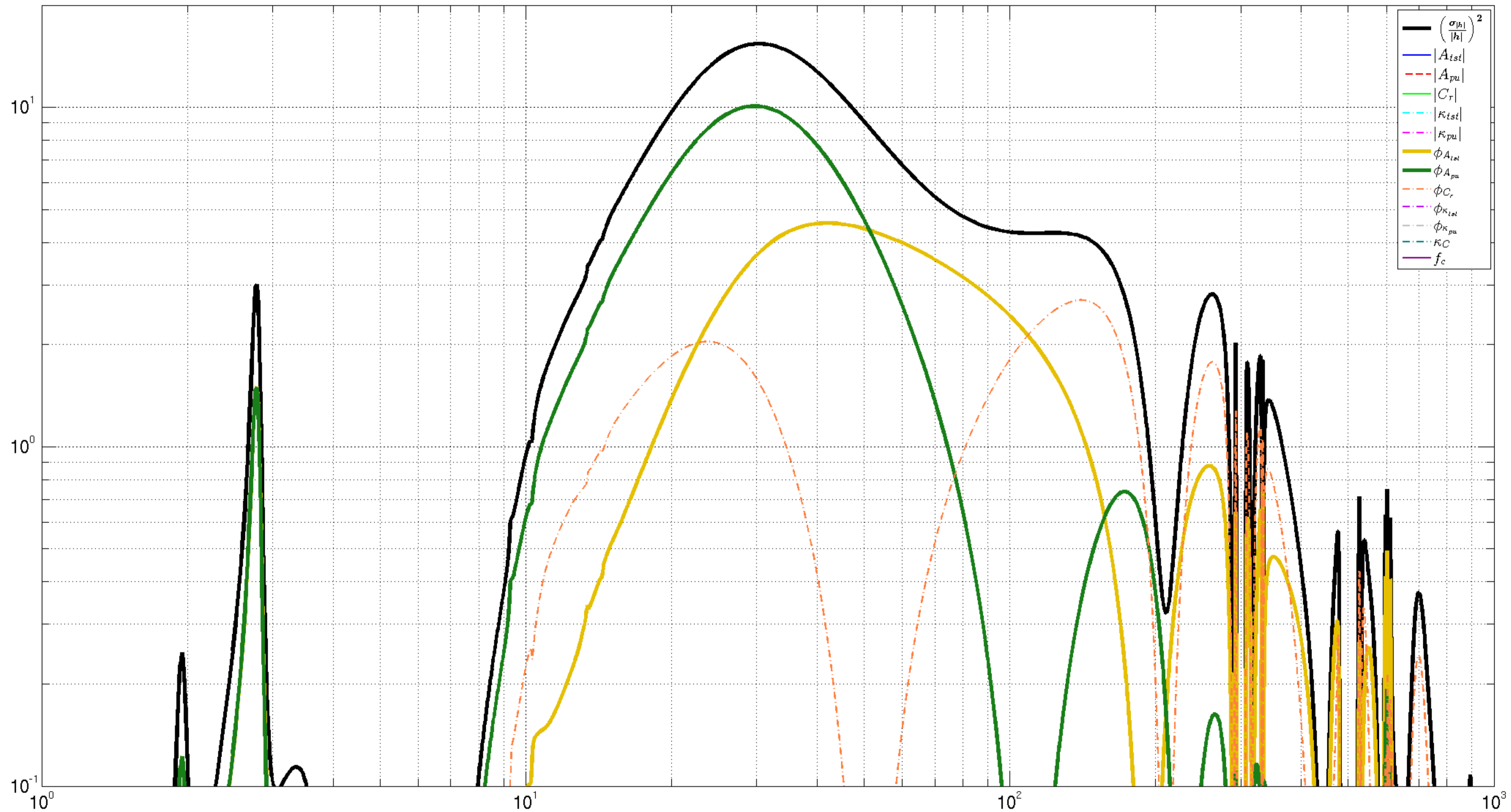
Squared Strain Magnitude Uncertainty Components \left(\frac{\partial|h|}{\partial(\text{legend})} \frac{1}{|h|}\right)^2 \sigma_{(\text{legend})}^2
