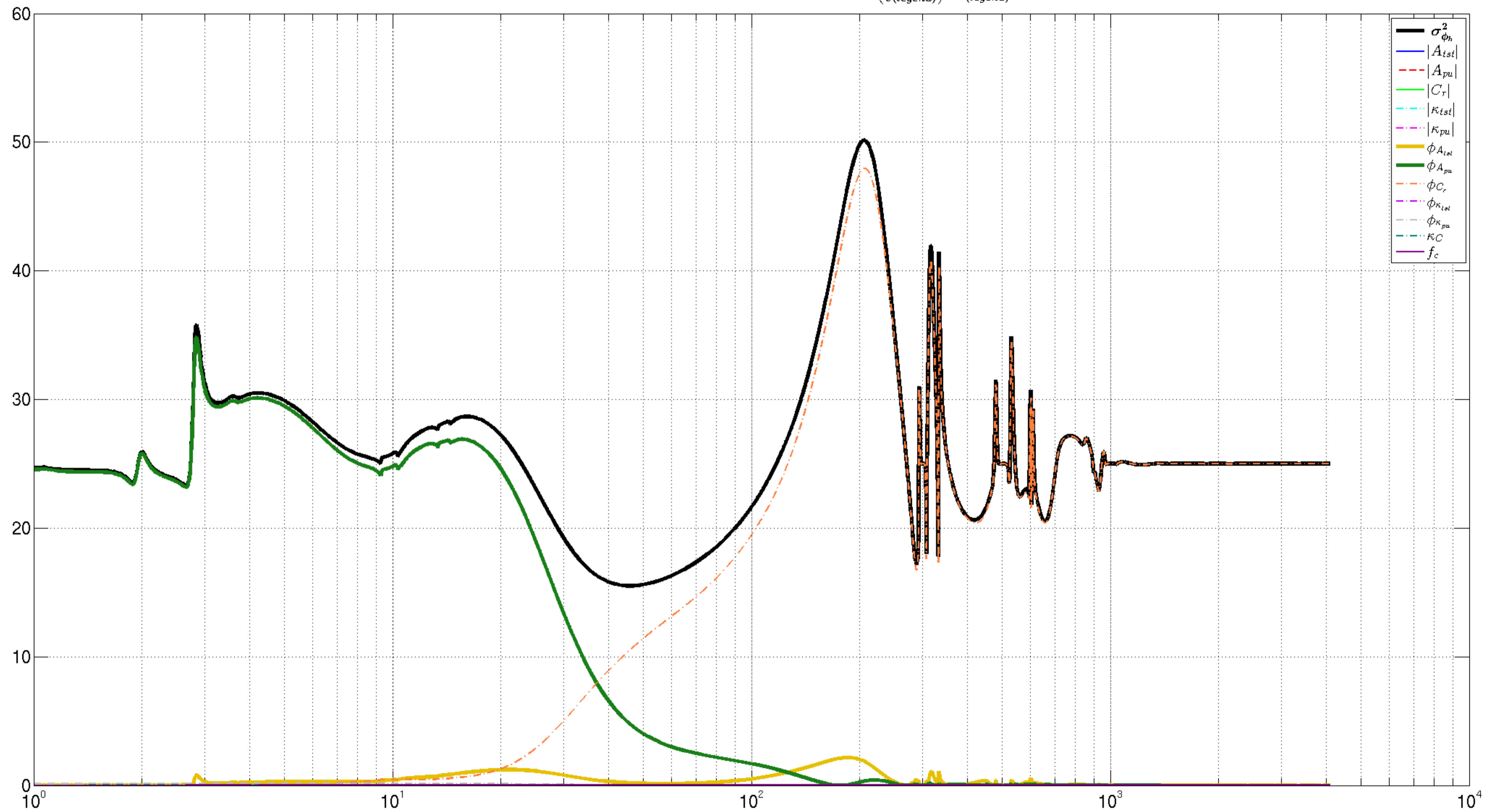
Squared Strain Phase Uncertainty Components \left(\frac{\partial \phi_h}{\partial(\text{legend})}\right)^2 \sigma_{(\text{legend})}^2
