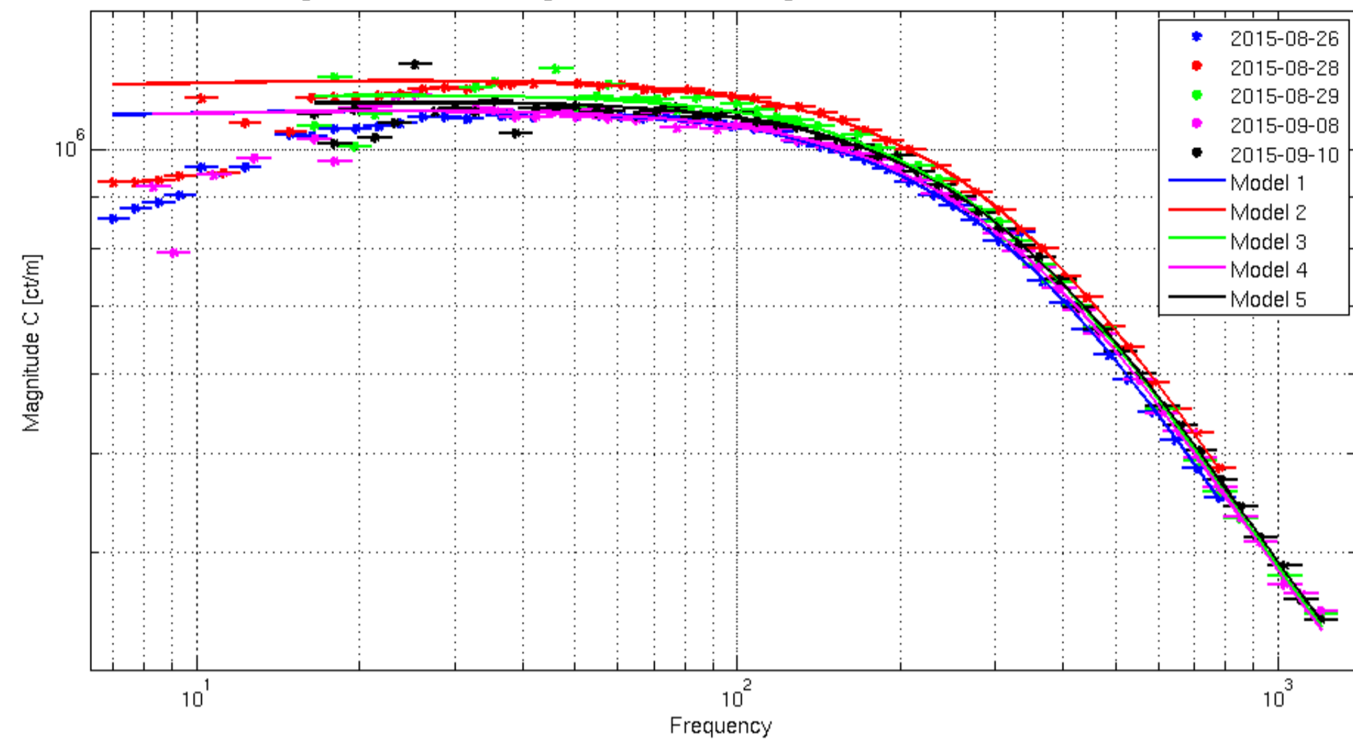
Magnitude Sensing - All 5 Sensing Function Measurements
