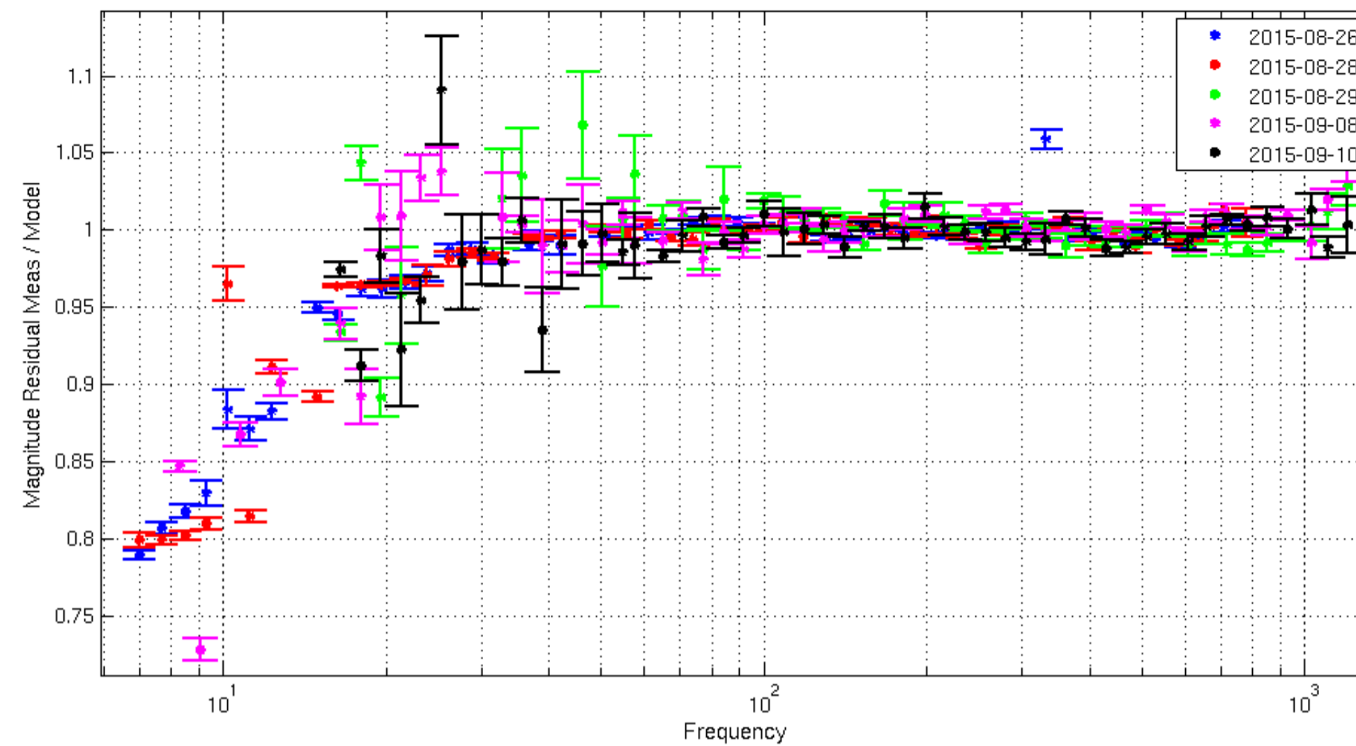
Magnitude Residuals (Meas / Model) with errorbars
