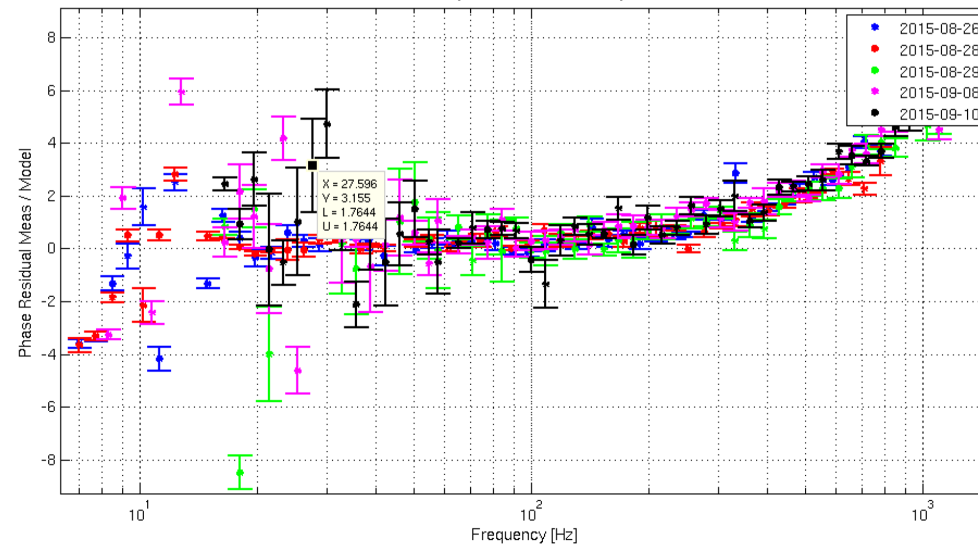
Phase Residuals (Meas / Model) with errorbars
