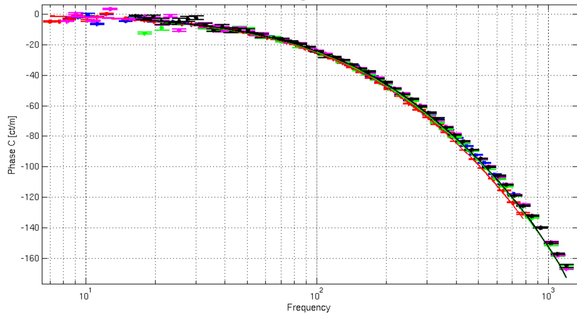
Phase Sensing Measurements
