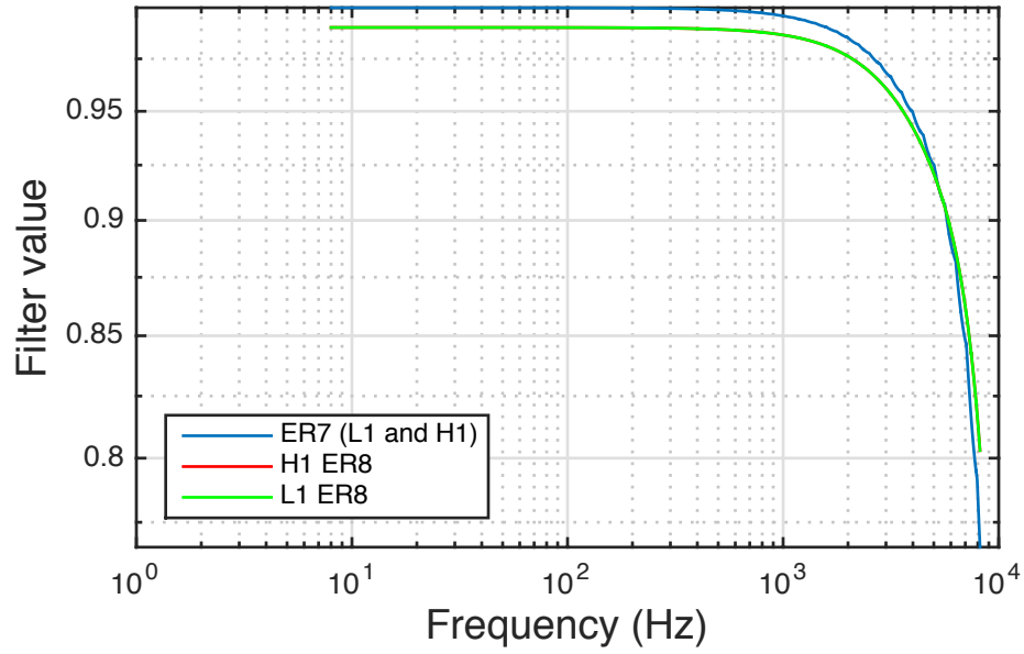
Magnitude response
