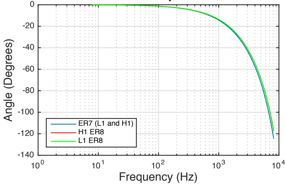
Phase response
