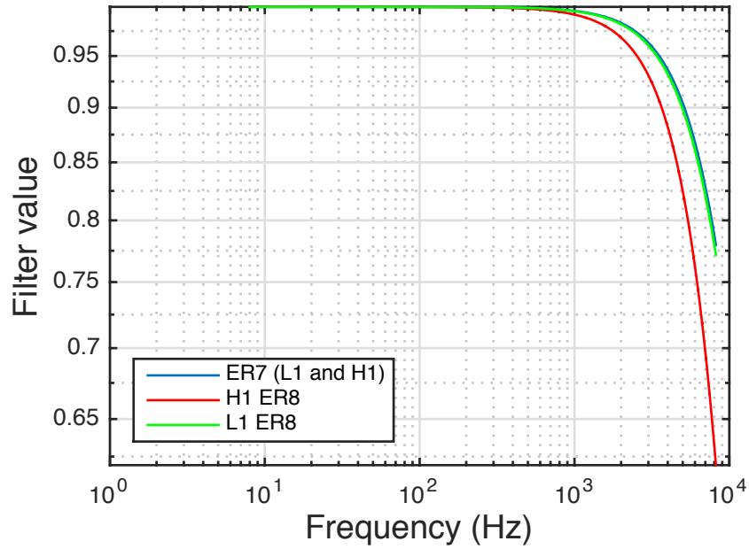
Magnitude response
