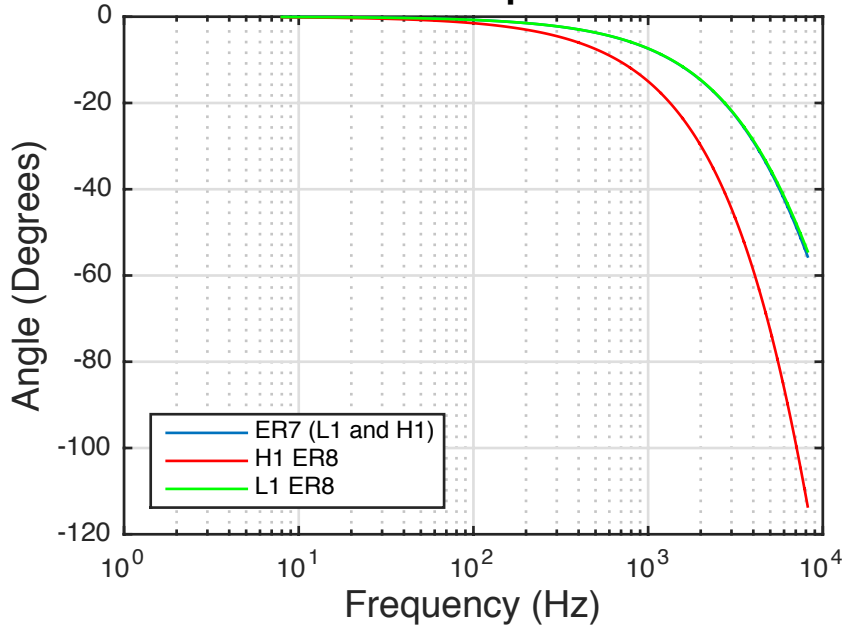
Phase response
