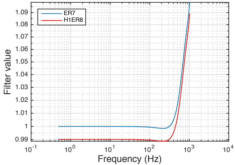
Magnitude response
