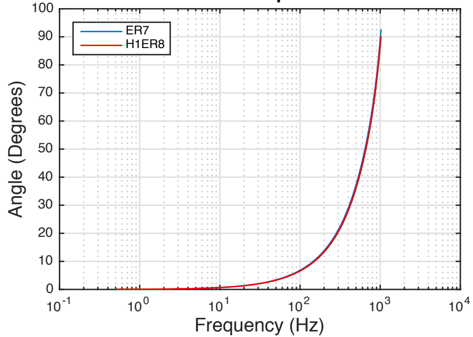
Phase response
