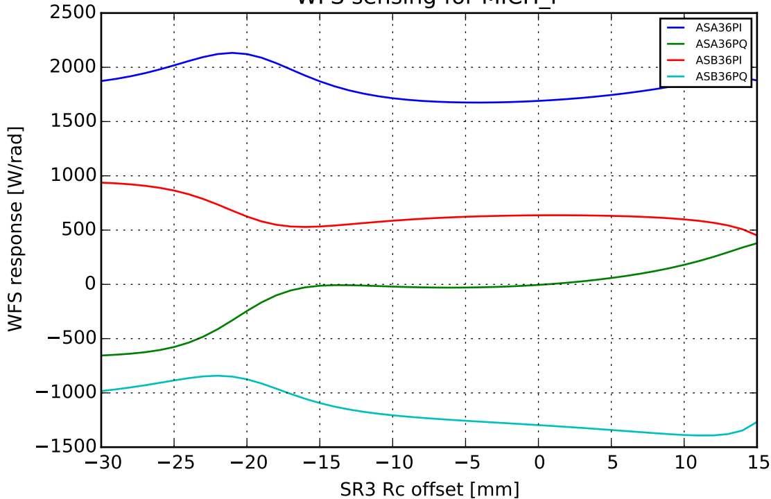
WFS sensing for MICH_P
