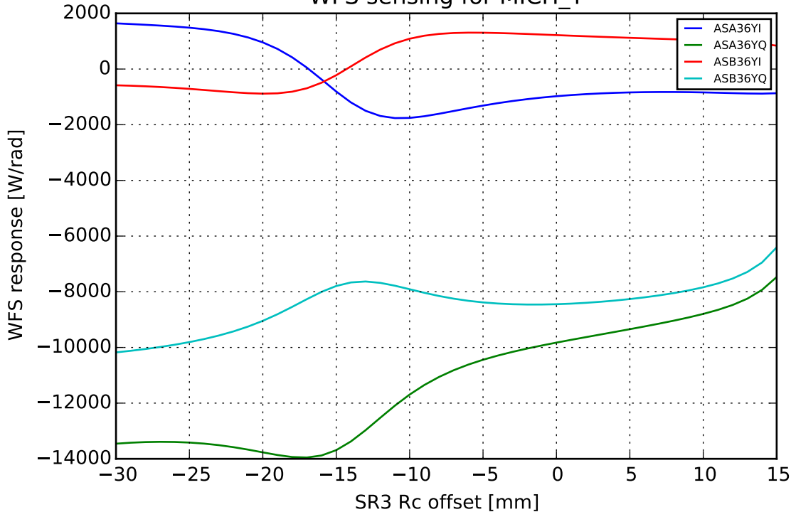
WFS sensing for MICH_Y
