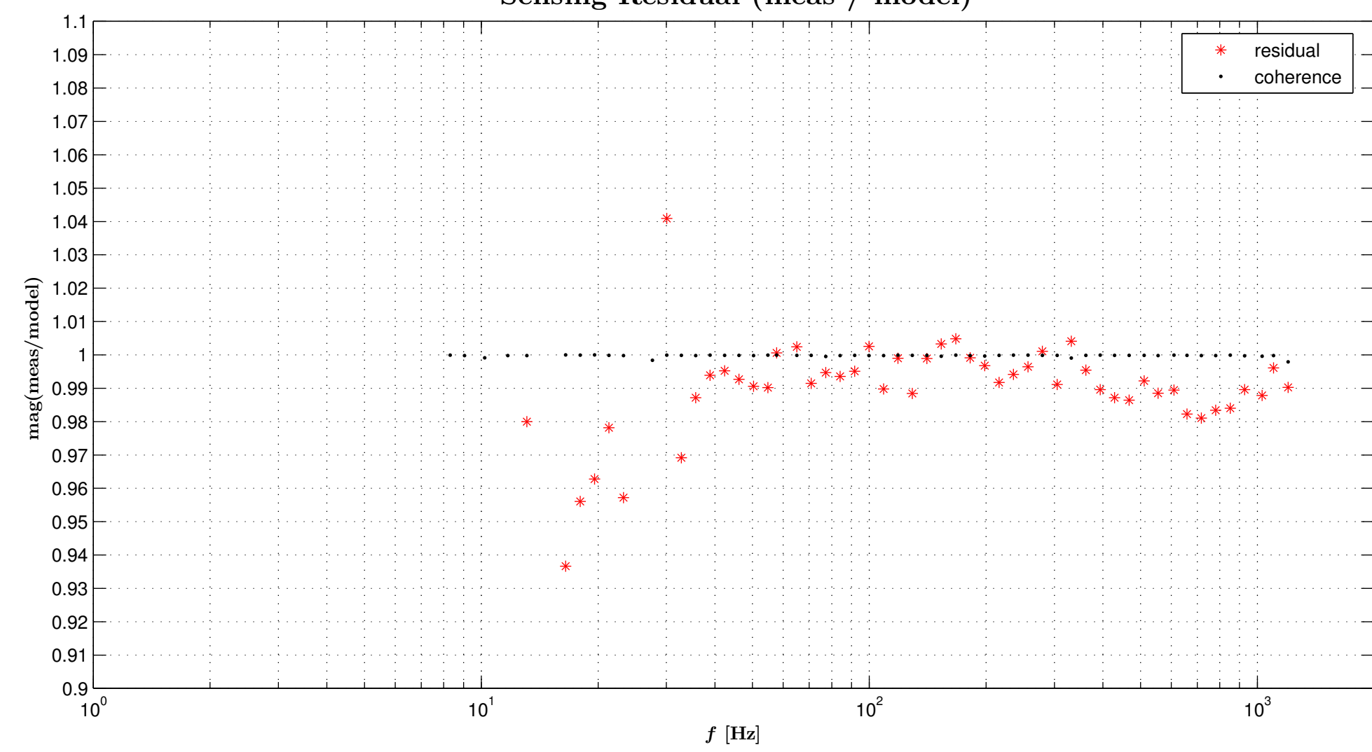
Sensing Residual (meas / model)
