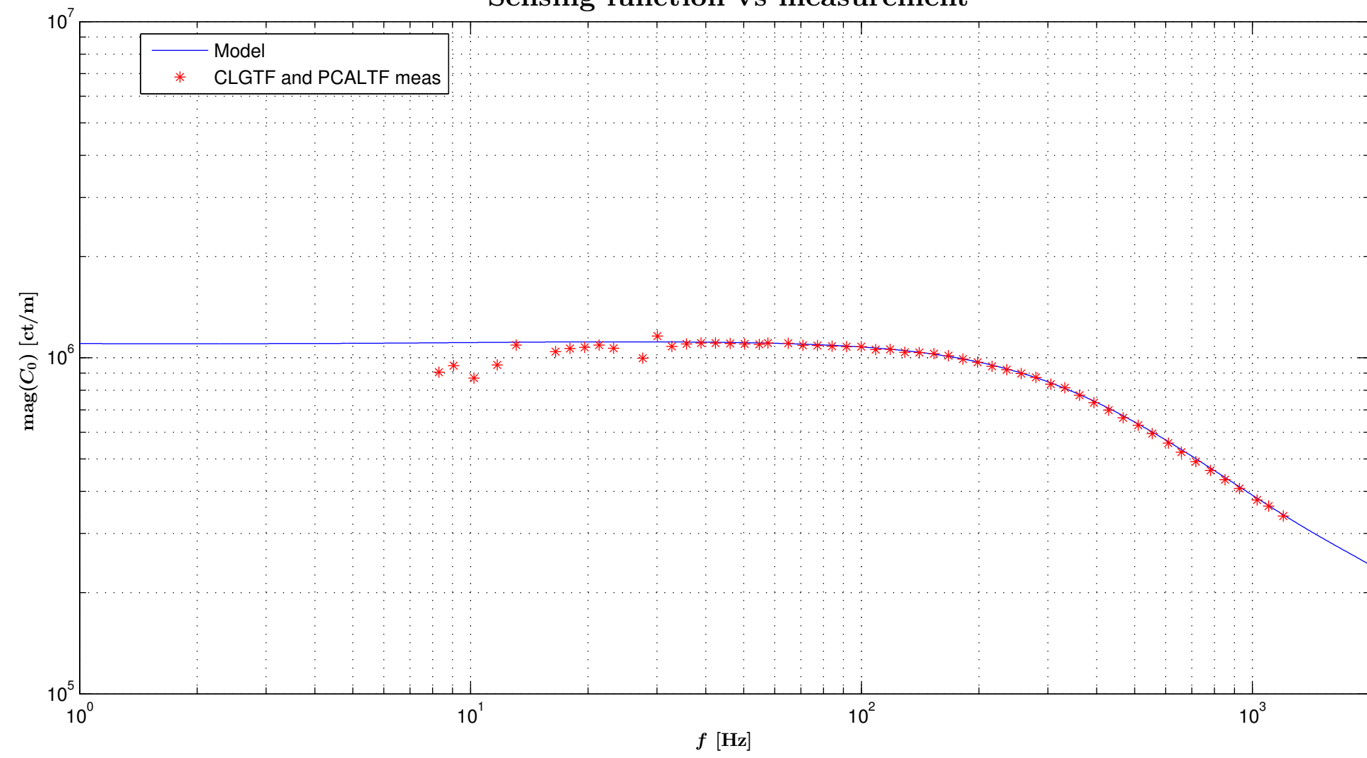
Sensing function vs measurement
