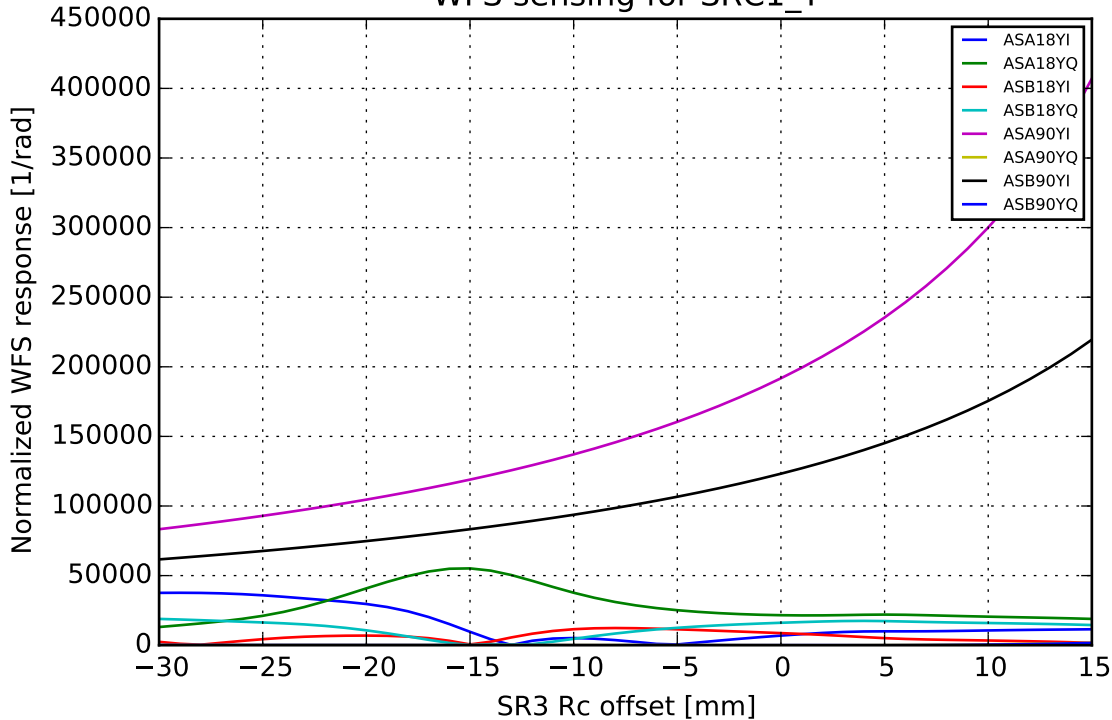
WFS sensing for SRC1_Y
