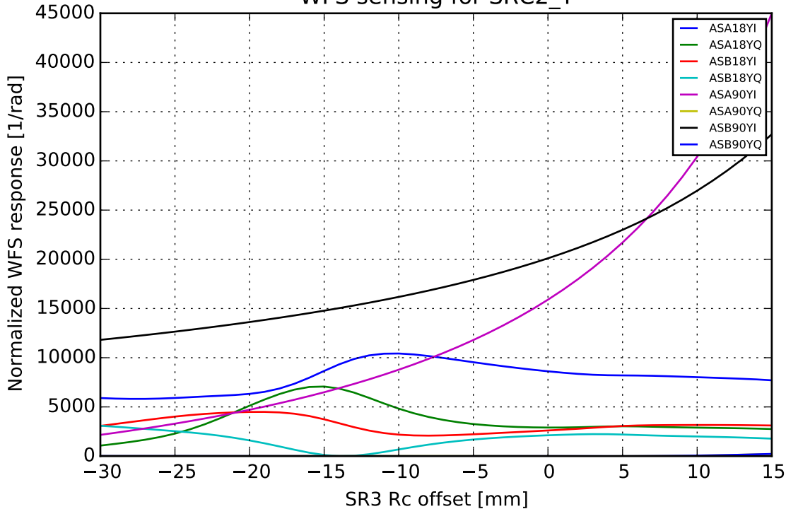
WFS sensing for SRC2_Y
