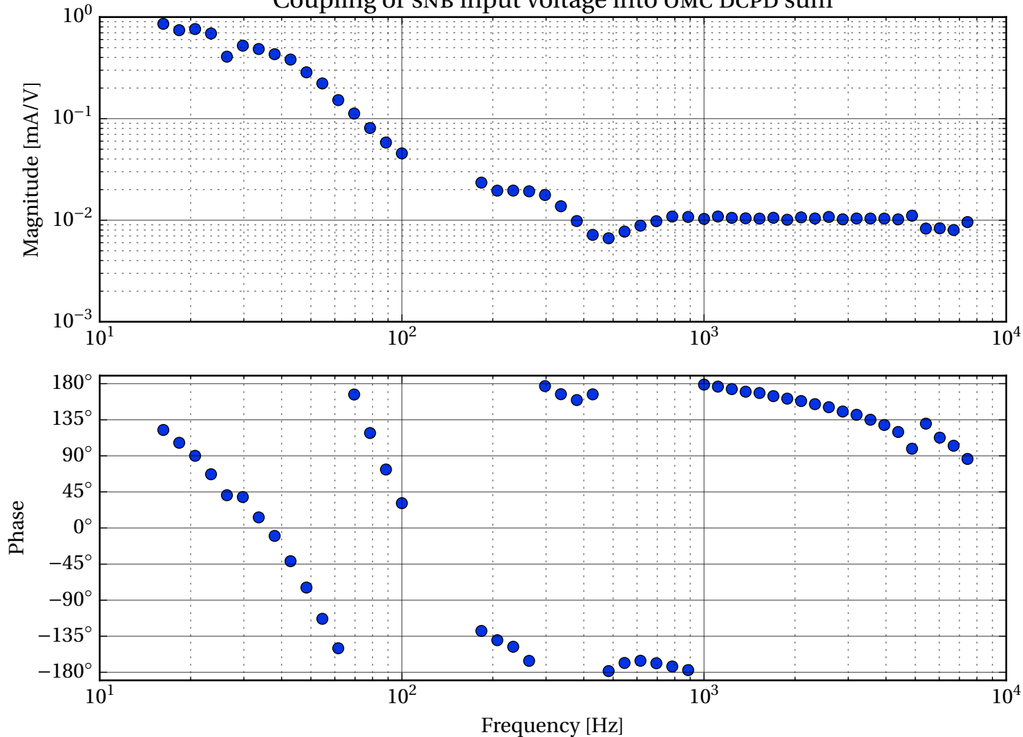
Coupling of snb input voltage into OMC DCPD sum
