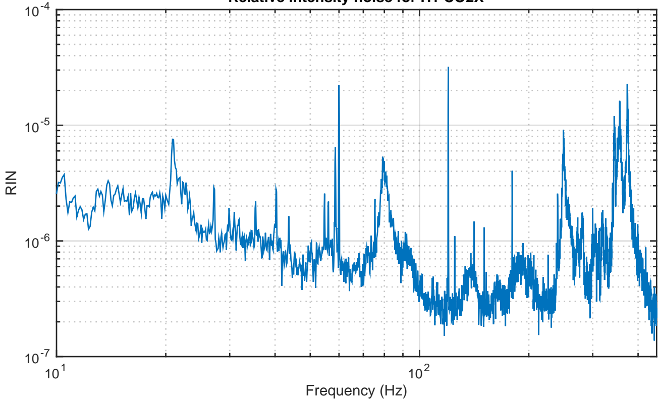
Relative intensity noise for H1 CO2X
