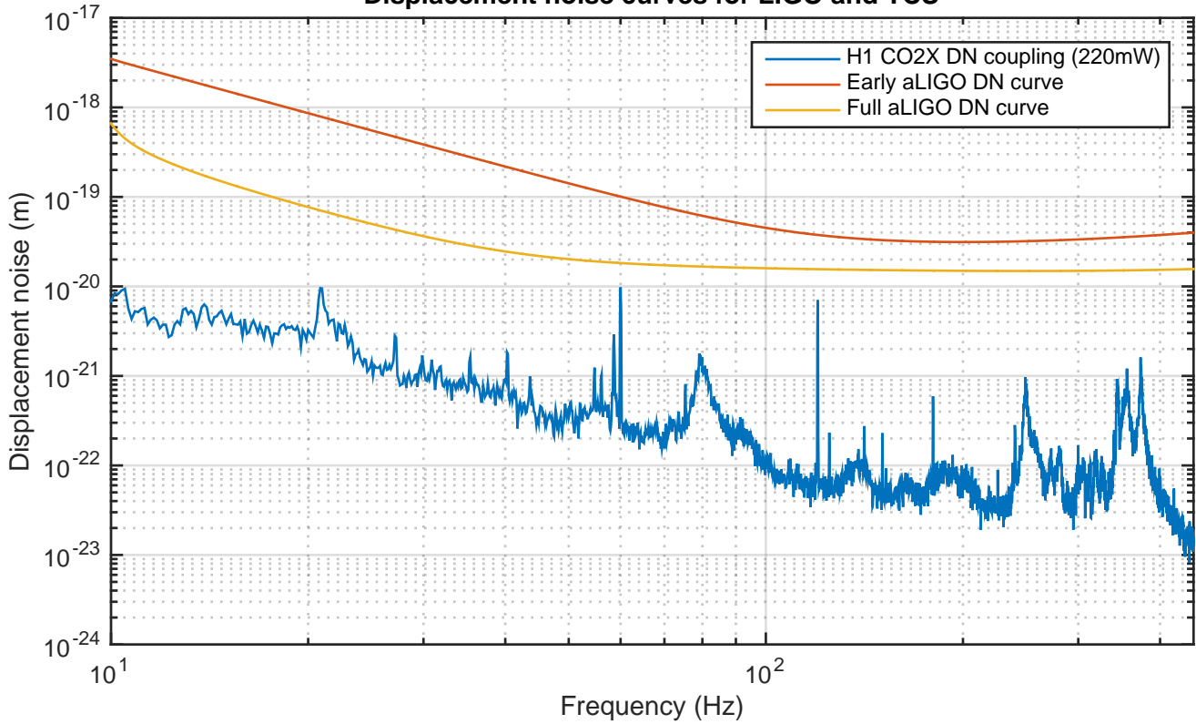
Displacement noise curves for LIGO and TCS
