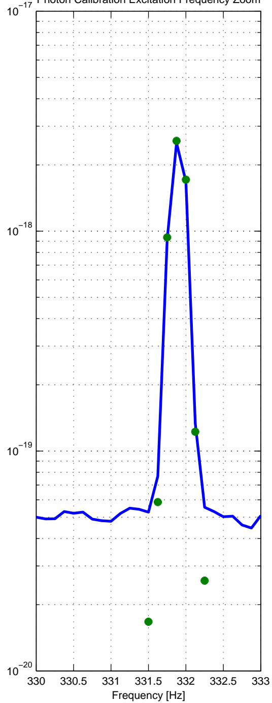
H1 Displacement Sensivity, Oct 01 2015 01:30:43 UTC Photon Calibration Excitation Frequency Zoom
