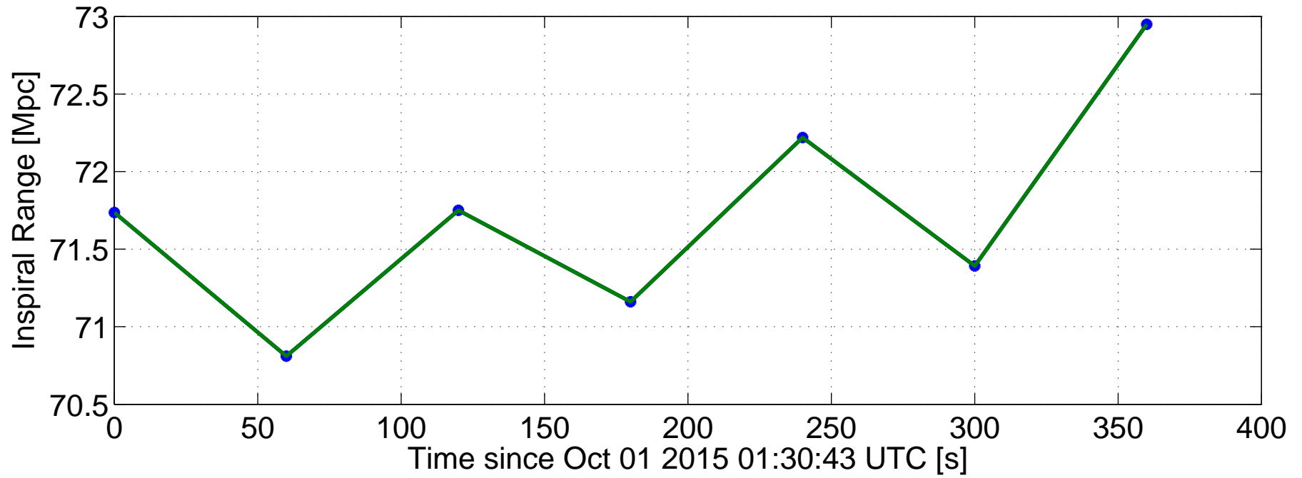
H1:DMT-SNSH_EFFECTIVE_RANGE_MPC.mean,m-trend
