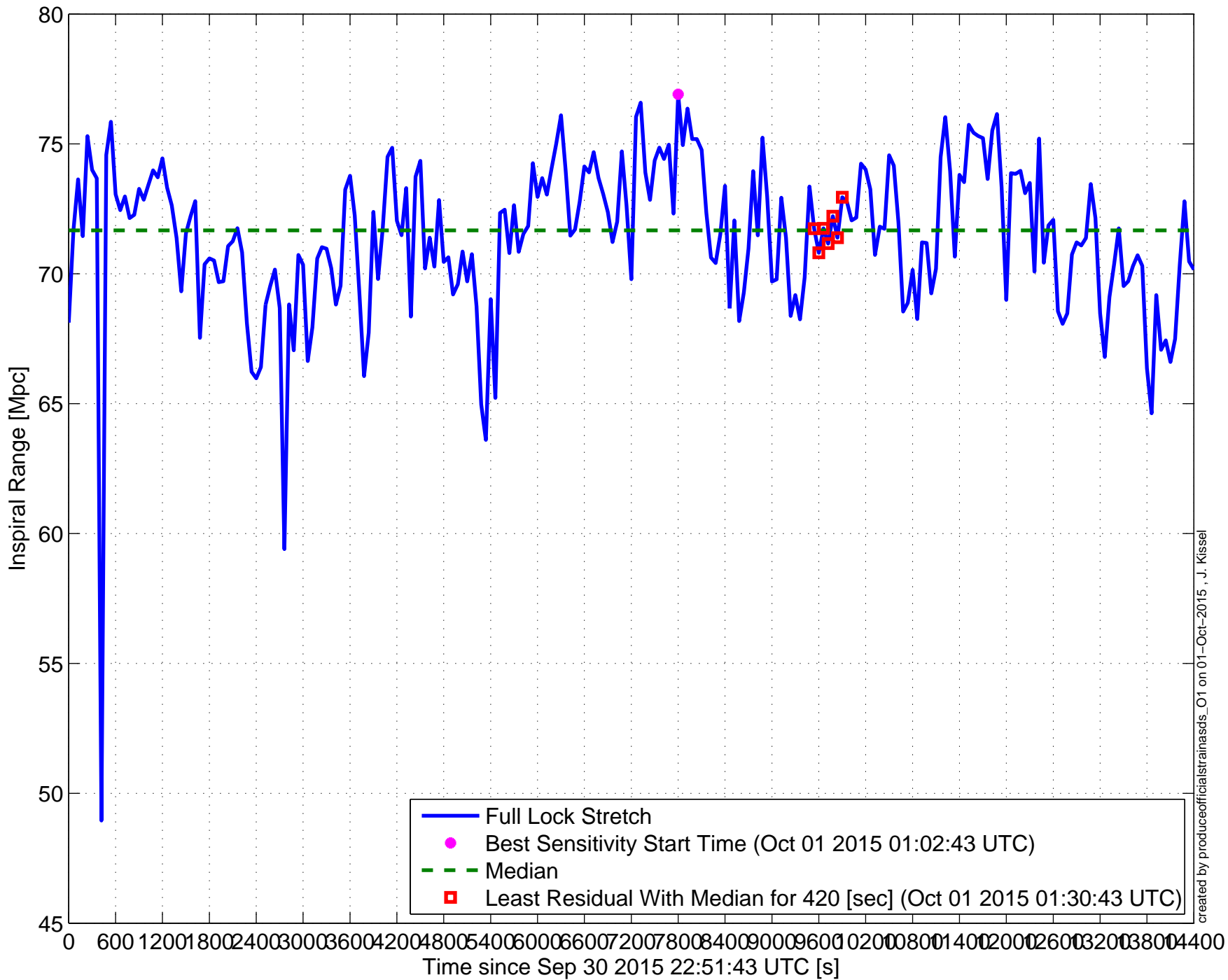
H1:DMT-SNSH_EFFECTIVE_RANGE_MPC.mean,m-trend
