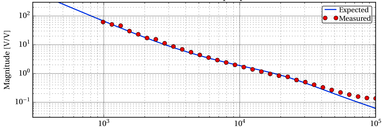
CARM OLTF, 23 W input power
