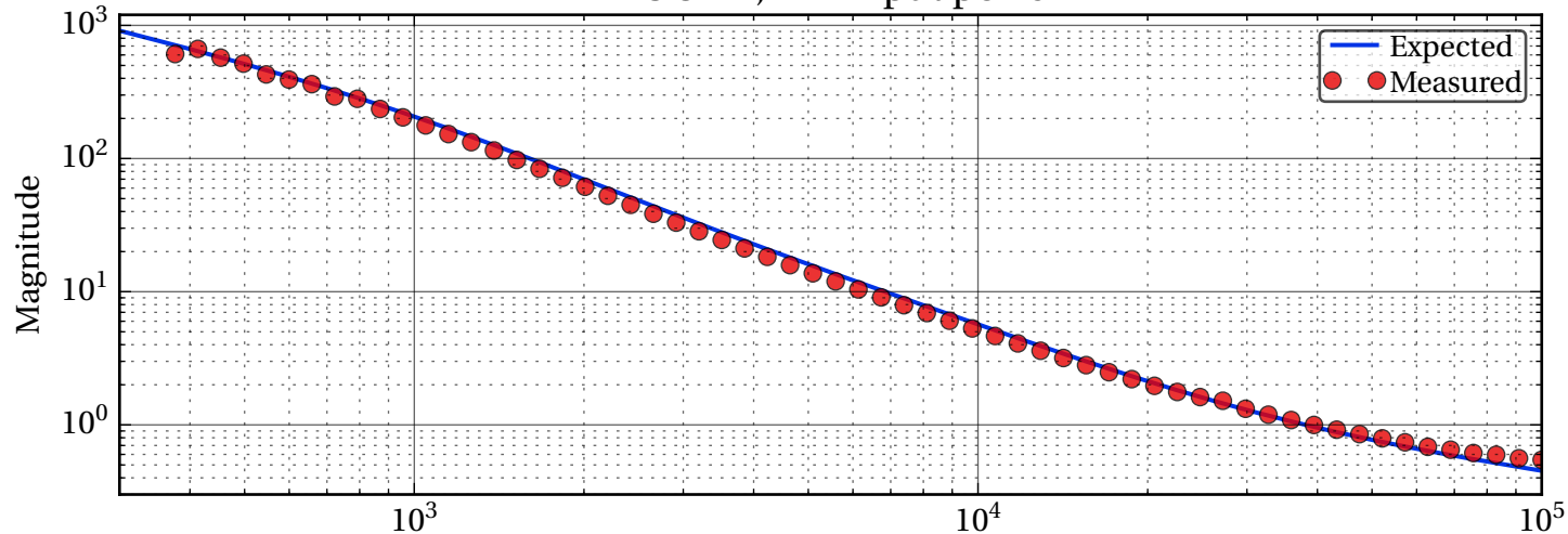
IMC OLTF, 2 W input power
