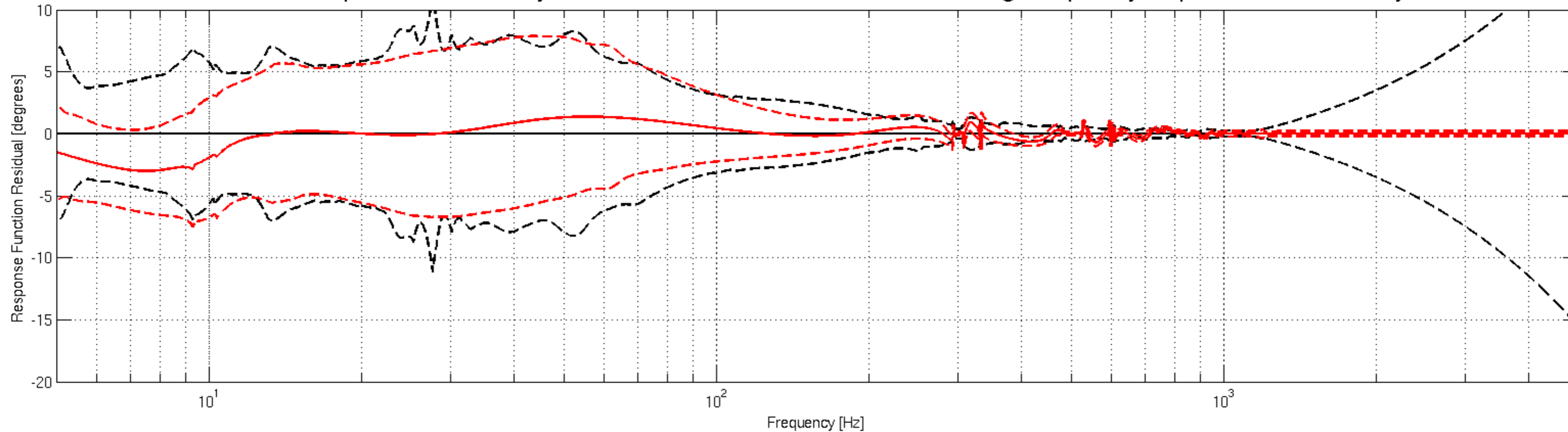
Phase Response Function Systematics / Nominal Residuals -- Including Frequency Dependent Uncertainty
