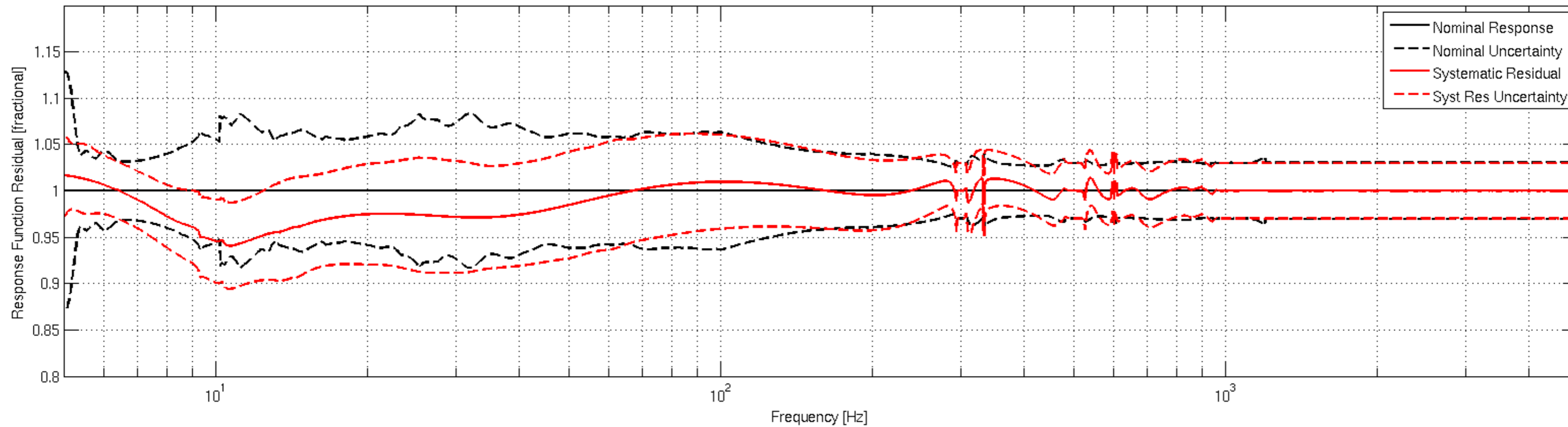
Magnitude Response Function Systematics / Nominal Residuals -- Including Frequency Dependent Uncertainty
