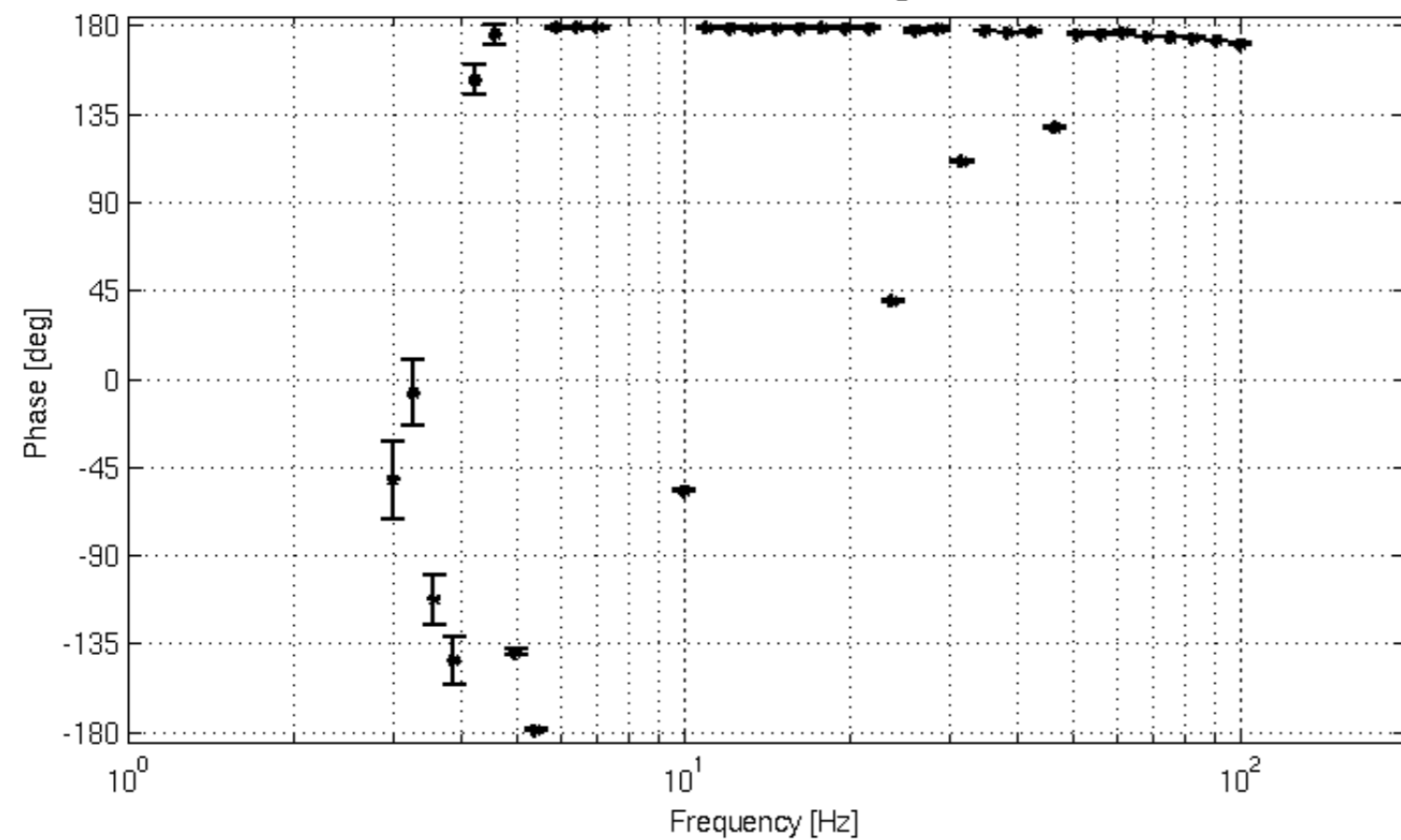
L1 Actuation Phase Weighted Mean
