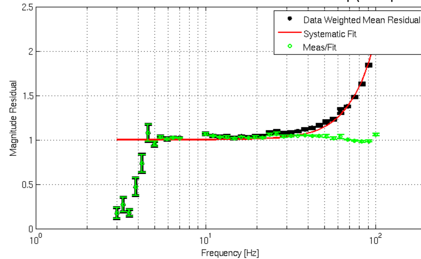
L1 Magnitude Meas/Fit Residual -- Fit: Zero Pair = 12.00 * \text{Exp}(+i * \pi/180 * 41.00) [Hz]
