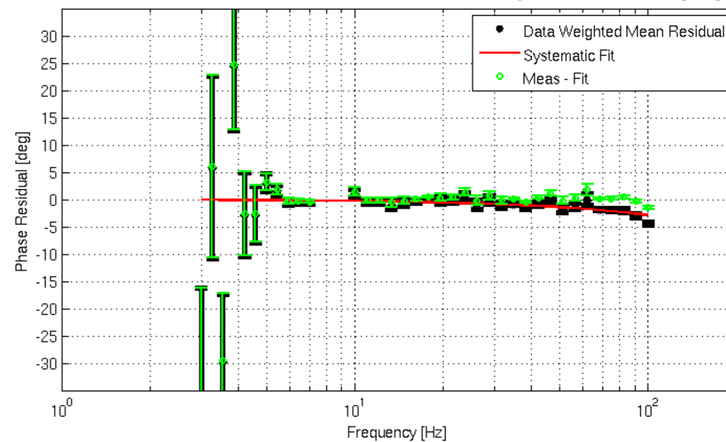
L1 Phase Meas/Fit Residual -- Fit: Delay = 79.900000 [us]
