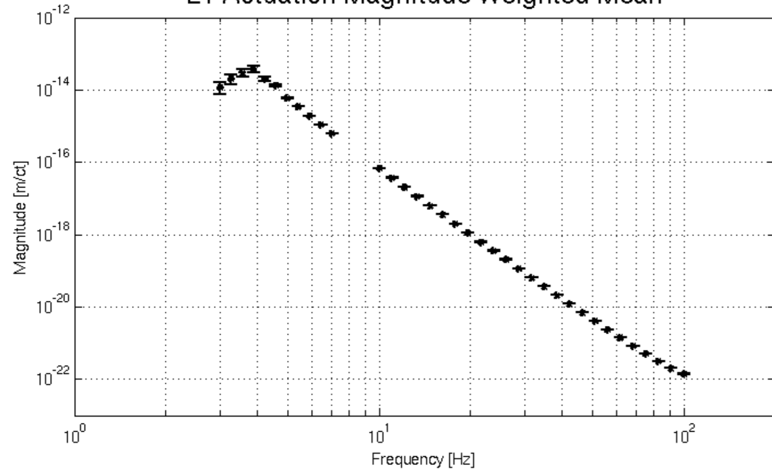
L1 Actuation Magnitude Weighted Mean
