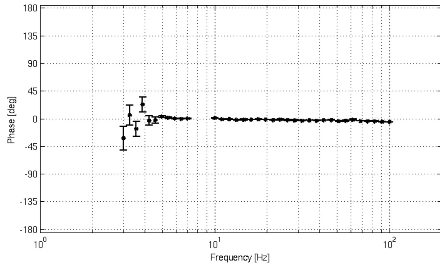
L2 Actuation Phase Weighted Mean
