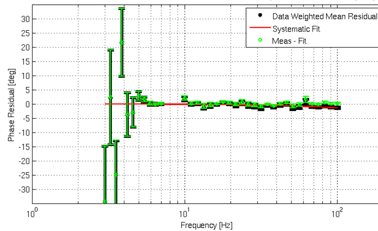
L2 Phase Meas/Fit Residual -- Fit: Delay = 39.000000 [us]
