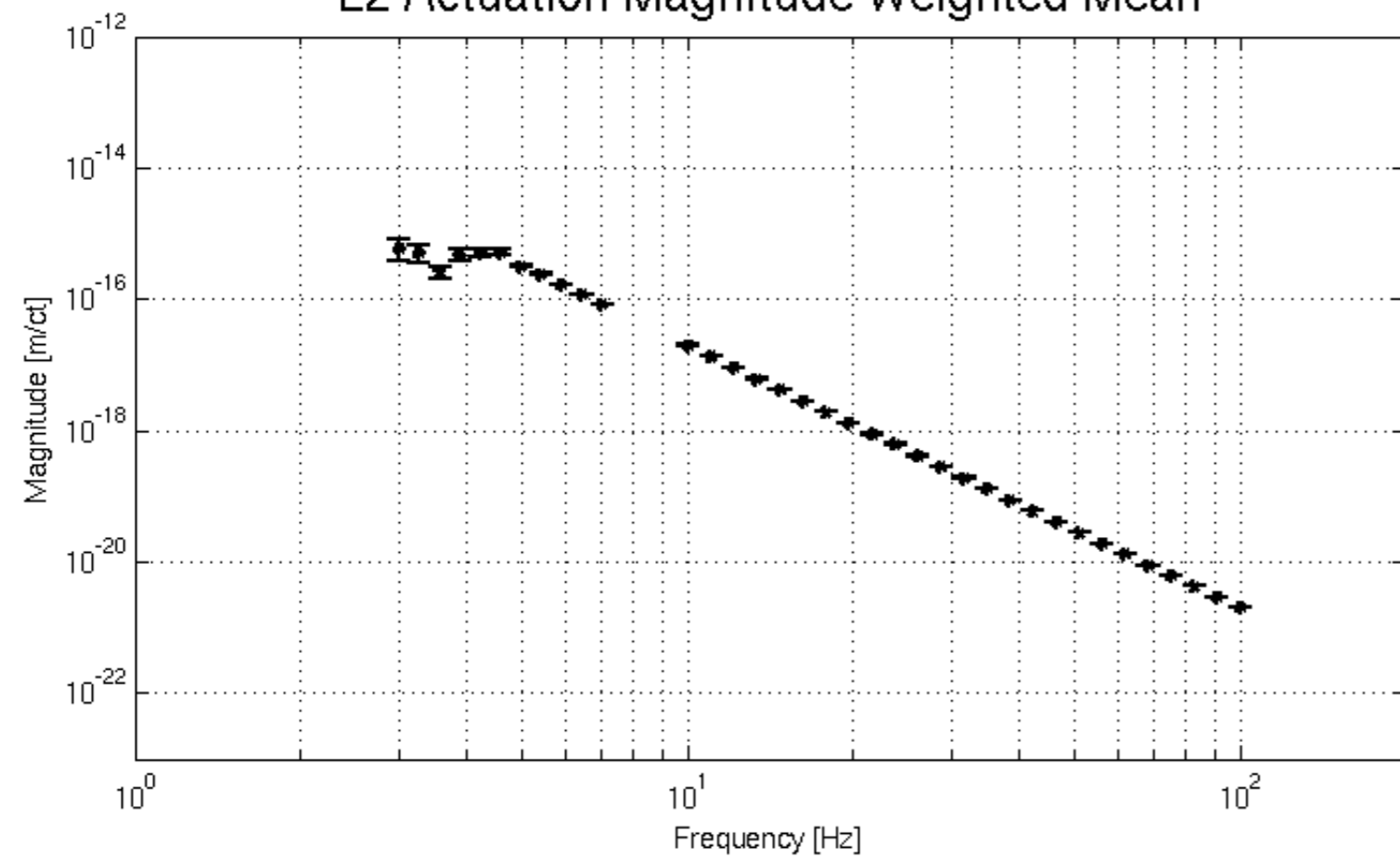
L2 Actuation Magnitude Weighted Mean
