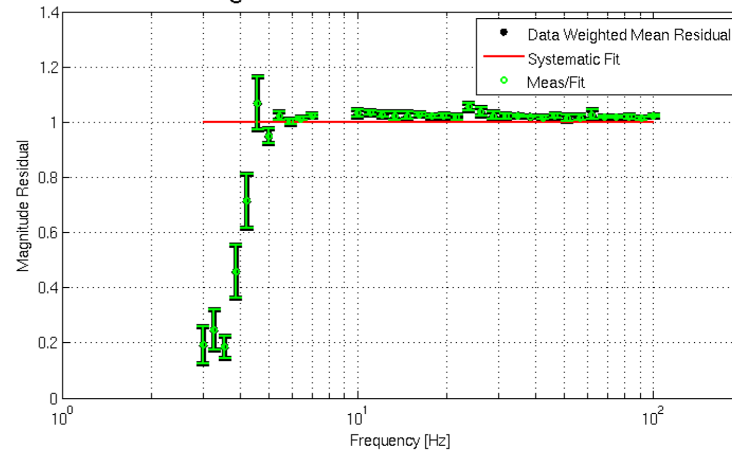
L2 Magnitude Meas/Fit Residual -- Fit: Flat
