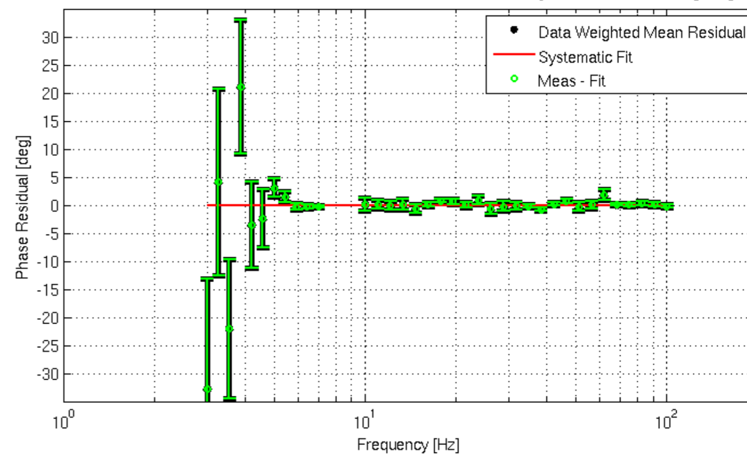
L3 Phase Meas/Fit Residual -- Fit: Delay = 0.000000 [us]
