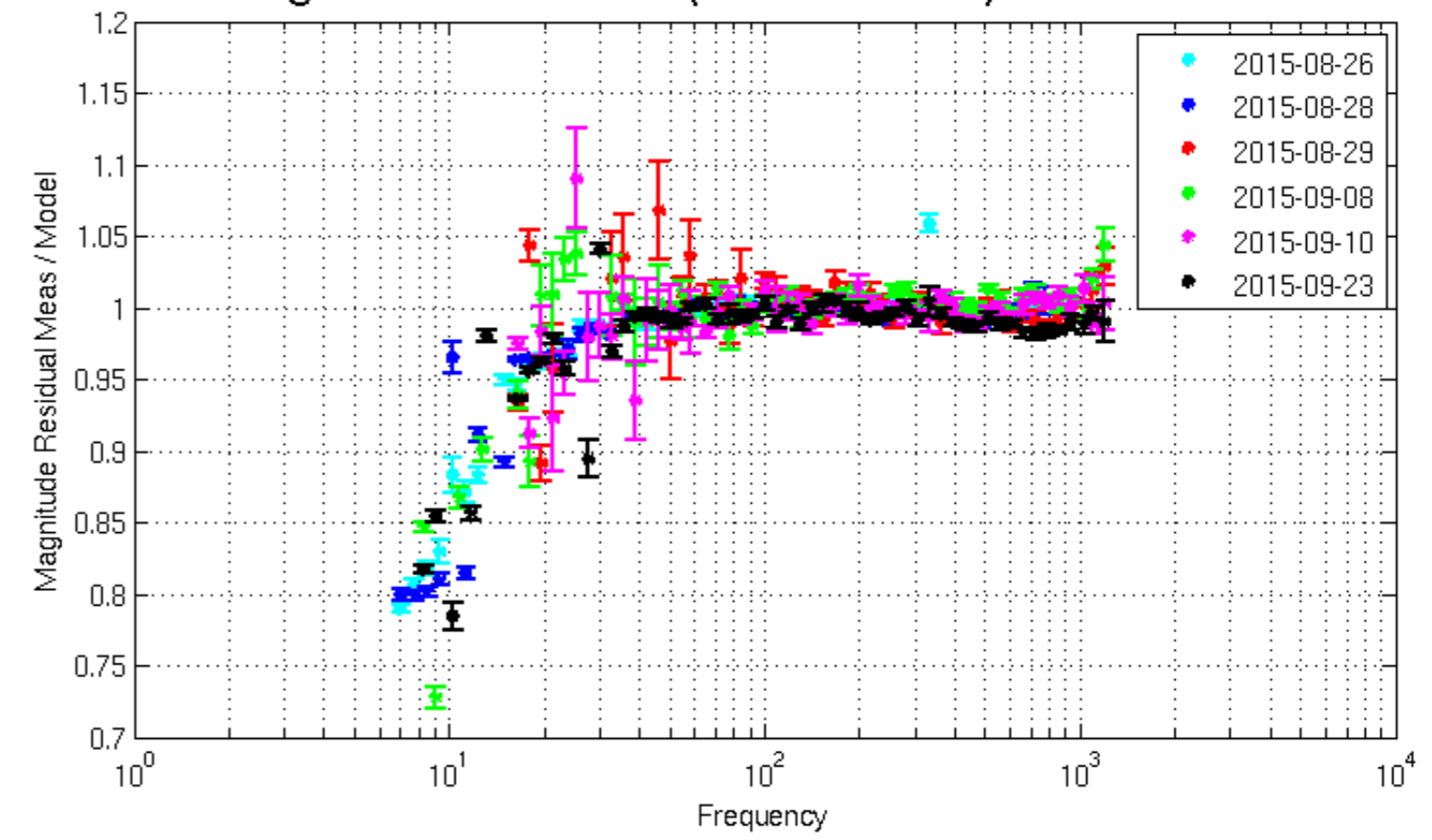
Magnitude Residuals (Meas / Model) with errorbars
