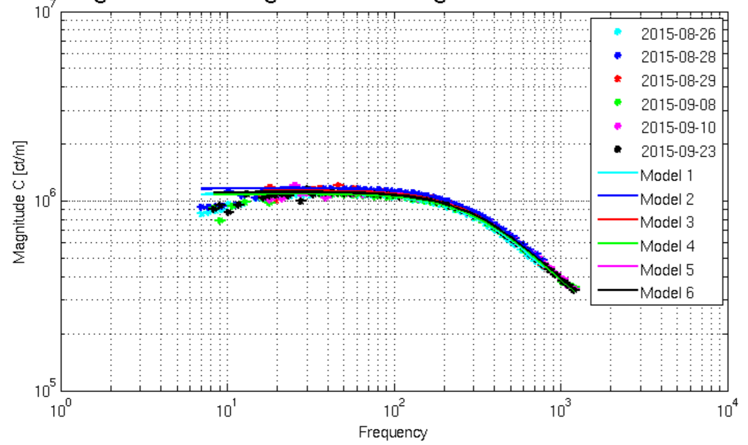
Magnitude Sensing - All 5 Sensing Function Measurements
