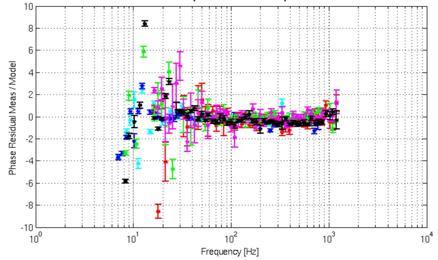
Phase Residuals (Meas / Model) with errorbars
