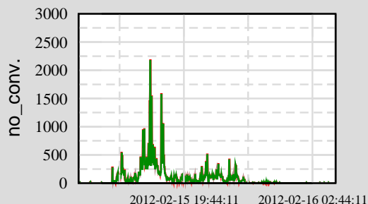
Ch 2: H0:PEM-LVEA_DST4_5
