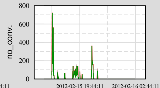
Ch 13: H0:PEM-LAB_DST2_5
