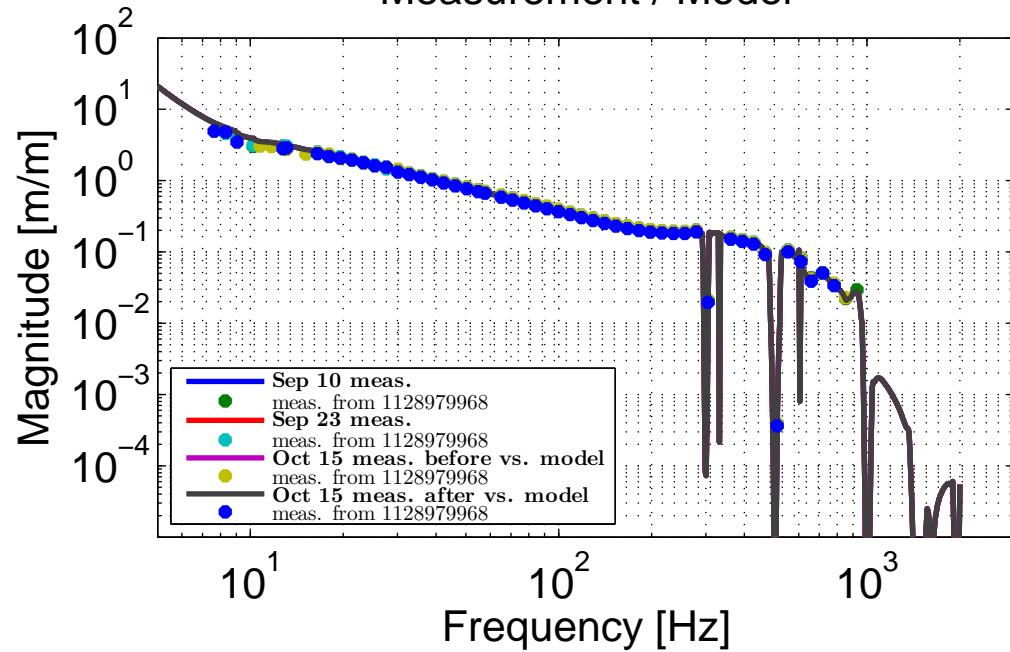
Latest DCC Pole Freq: 341 [Hz]
