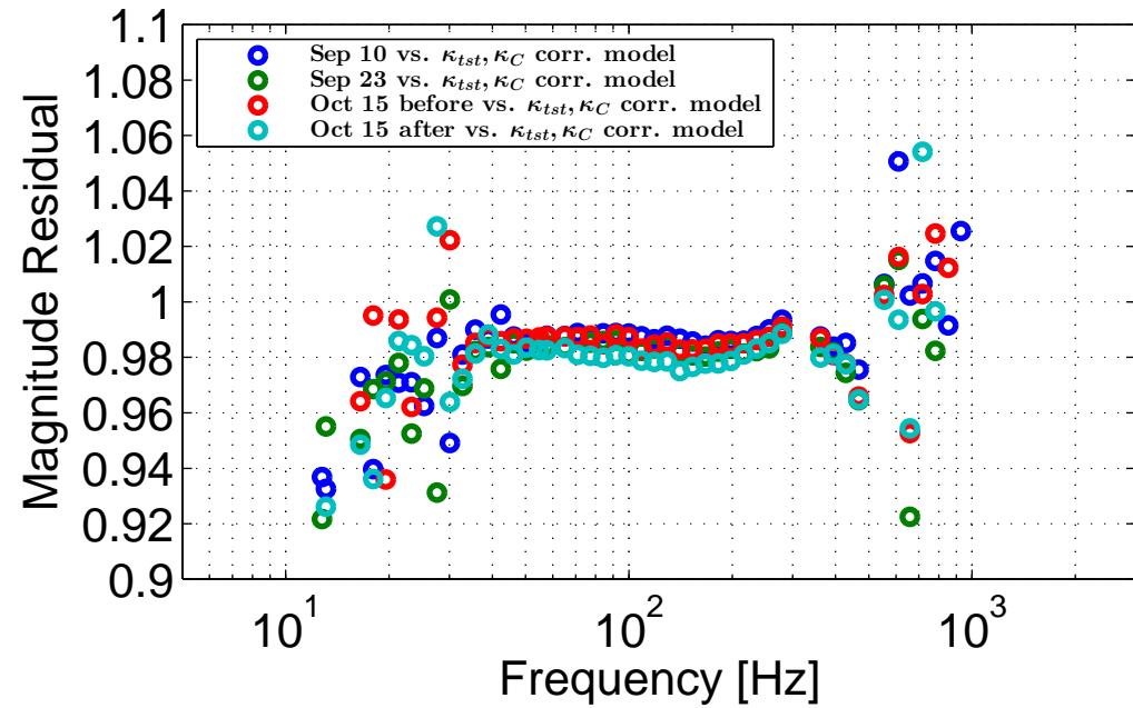
H1 DARM Open Loop Gain TF Comparison Meas. / KappaCorrectedModel
