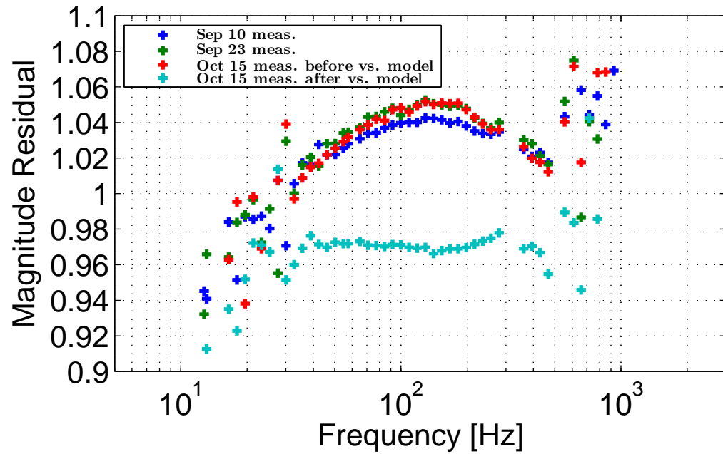
H1 DARM Open Loop Gain TF Comparison Measurement / Model
