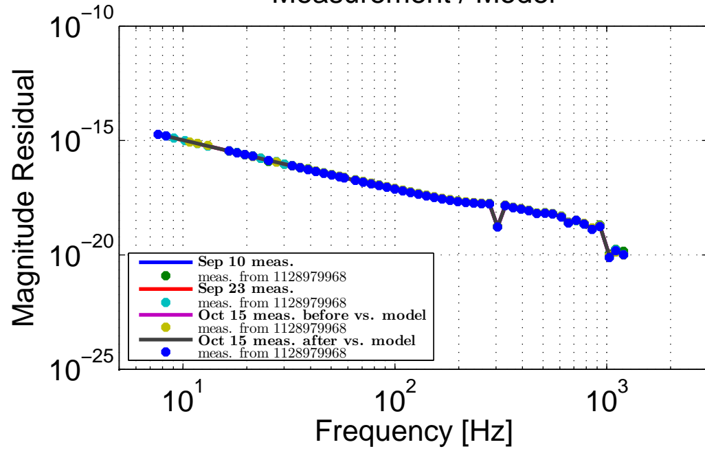
H1 Actuation Comparison Measurement / Model
