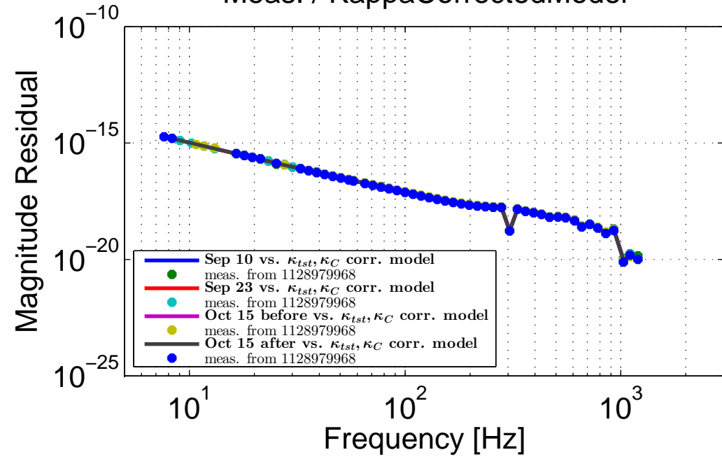
H1 Actuation Comparison Meas. / KappaCorrectedModel
