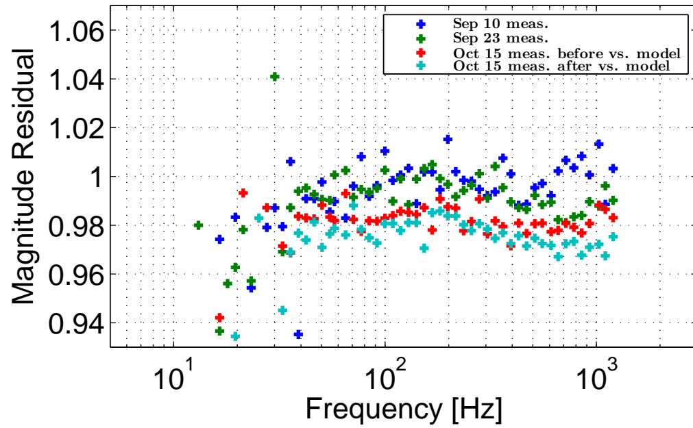
H1 Sensing Residual Measurement / Model
