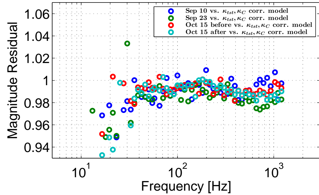
H1 Sensing Residual Meas. / KappaCorrectedModel
