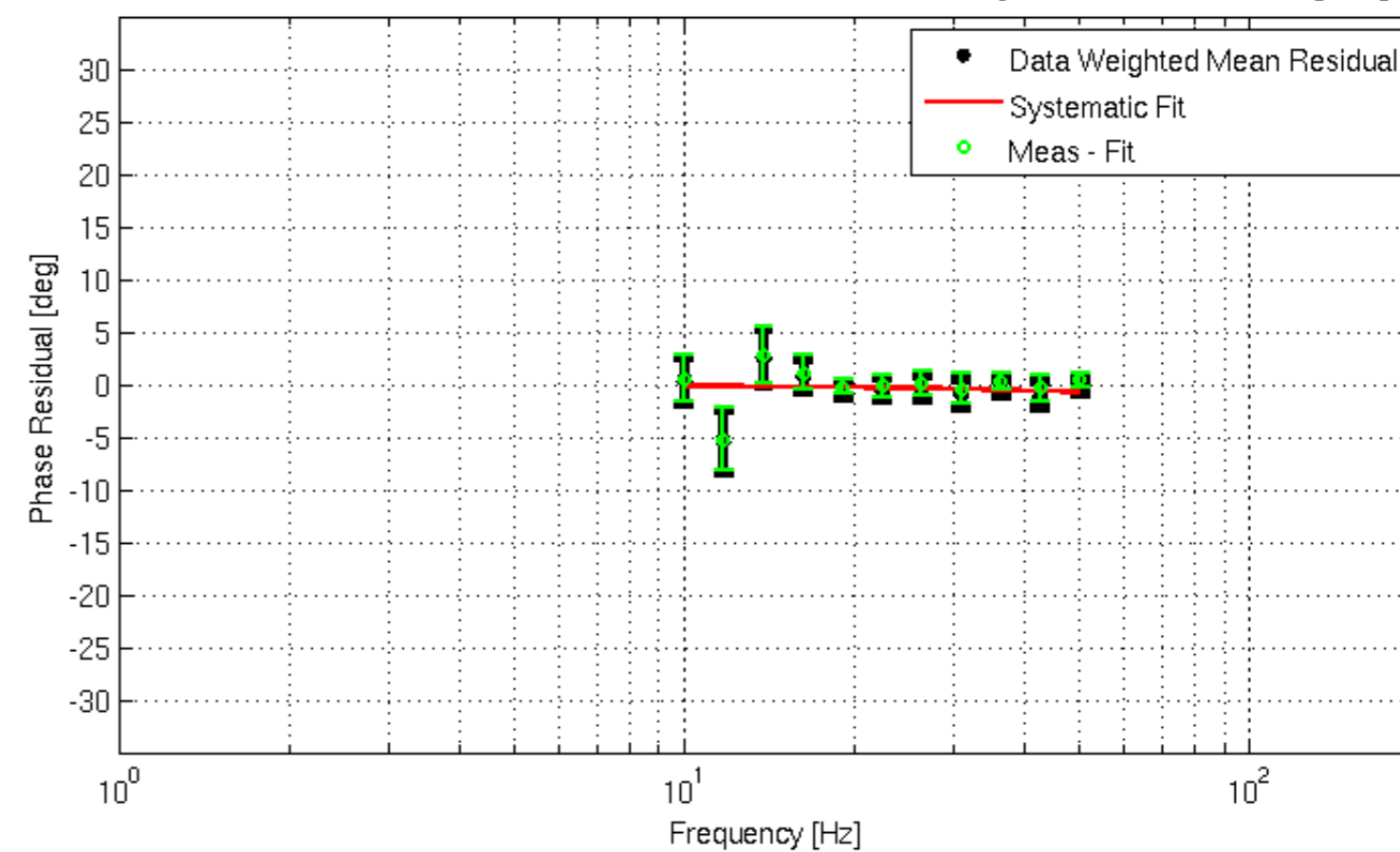
L1 Phase Meas/Fit Residual -- Fit: Delay = 39.200000 [us]
