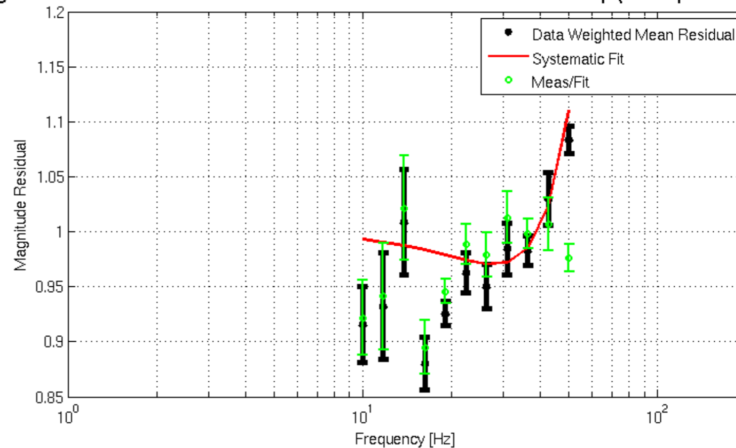
L1 Magnitude Meas/Fit Residual -- Fit: Zero Pair = 9.00 * Exp(+i * pi/180 * 52.00) [Hz]
