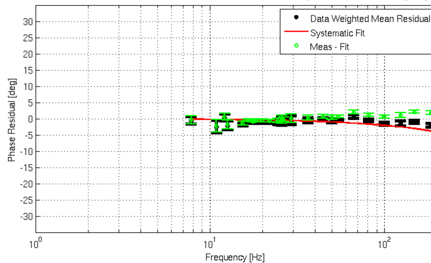
L2 Phase Meas/Fit Residual -- Fit: Delay = 57.500000 [us]
