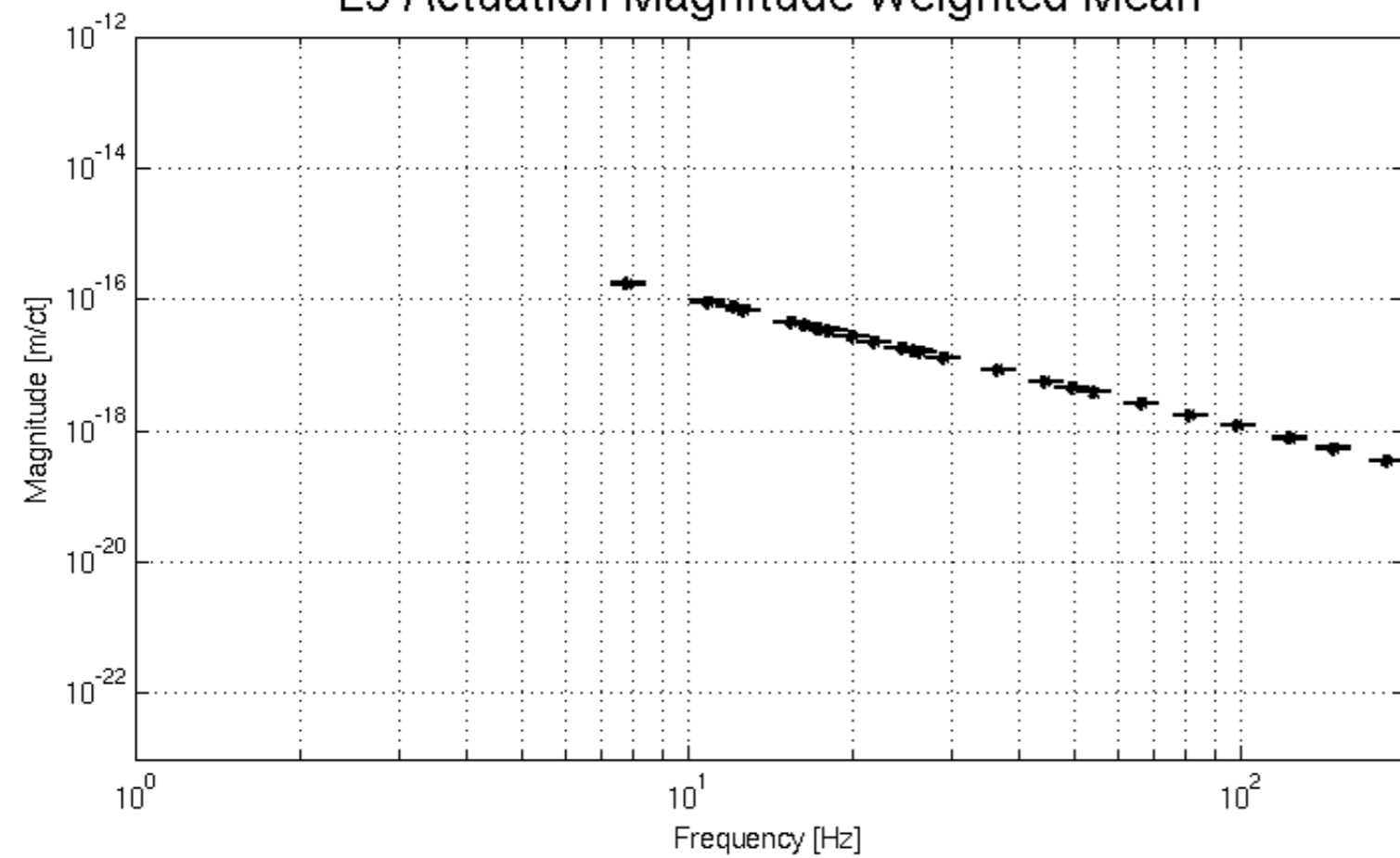
L3 Actuation Magnitude Weighted Mean
