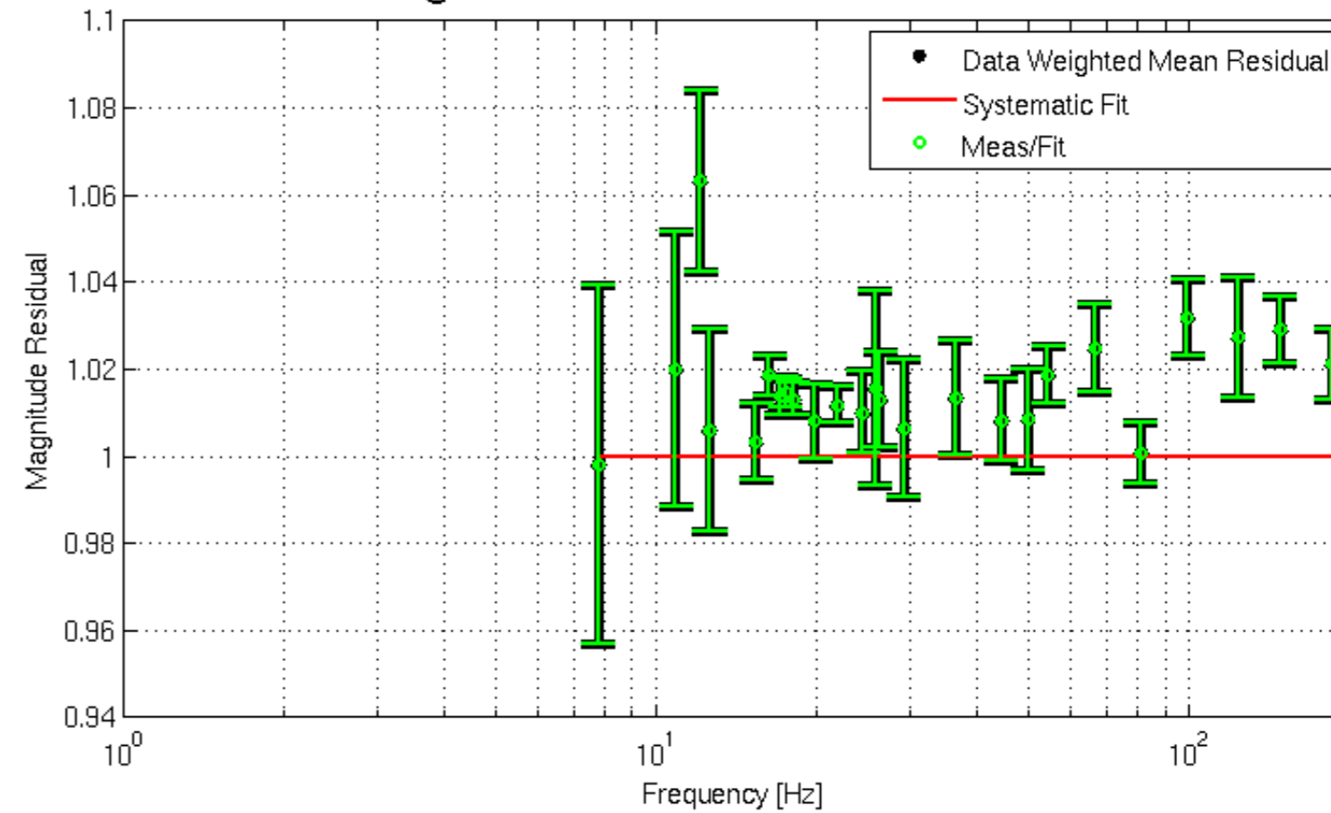
L3 Magnitude Meas/Fit Residual -- Fit: Flat
