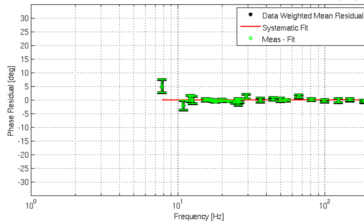
L3 Phase Meas/Fit Residual -- Fit: Delay = 1.200000 [us]
