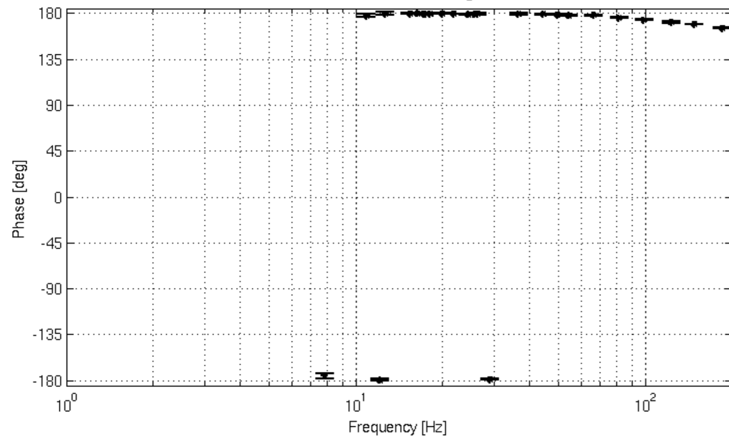
L3 Actuation Phase Weighted Mean
