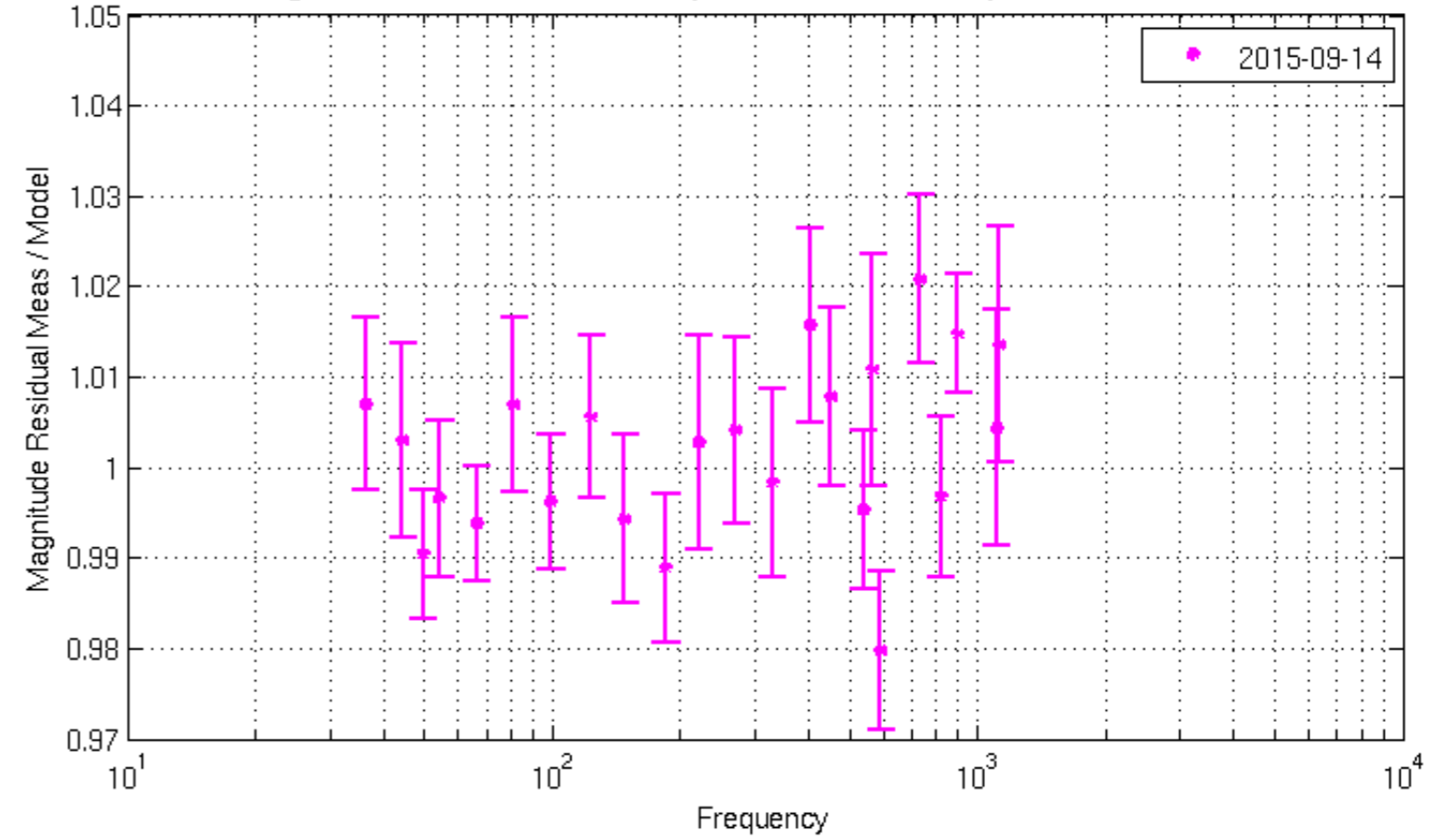
Magnitude Residuals (Meas / Model) with errorbars
