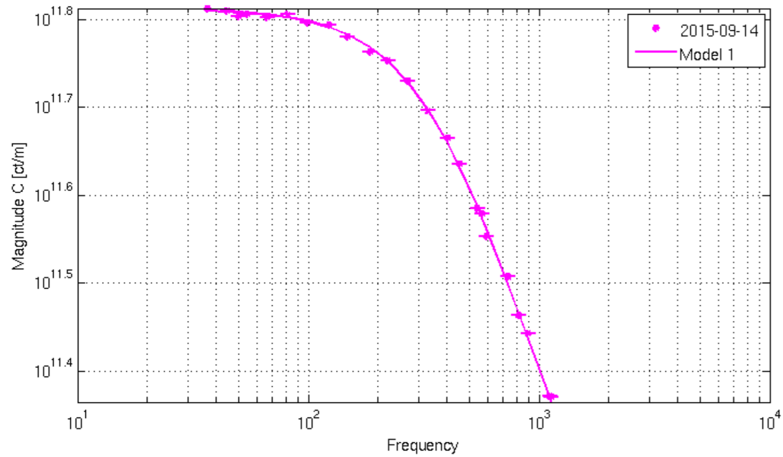
Magnitude Sensing - Sensing Function Measurement
