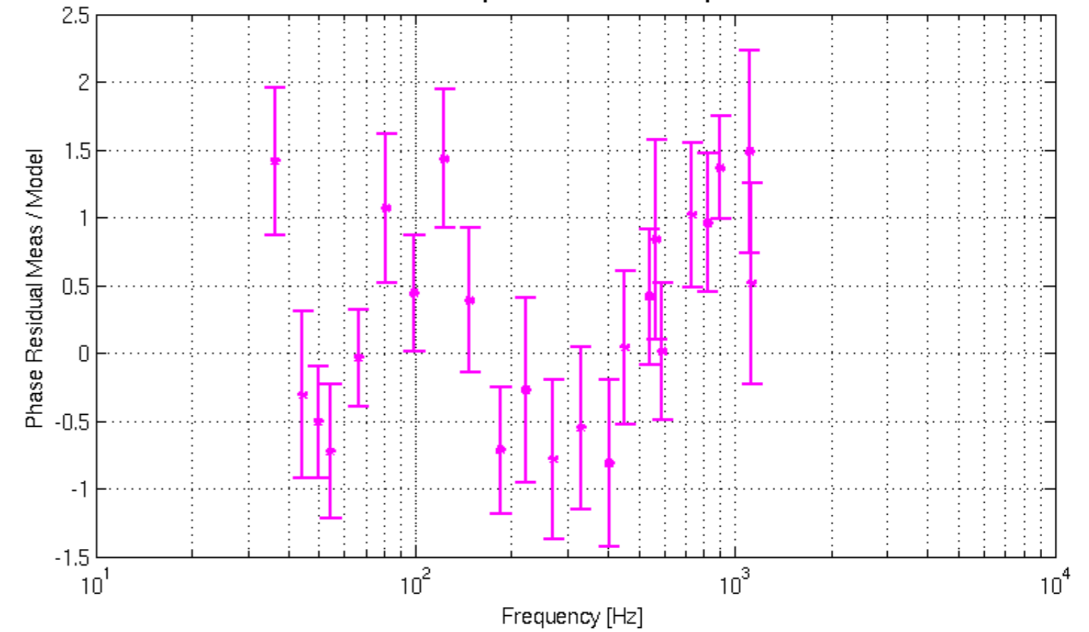
Phase Residuals (Meas / Model) with errorbars
