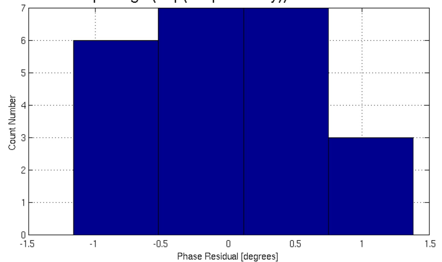
Phase Res -- Systematic: 180 / \pi * \text{Angle}(\text{Exp}(i * 2 * \pi * f * \text{delay})) -- Advance: 2.4e-06 -- Std: 0.722 deg
