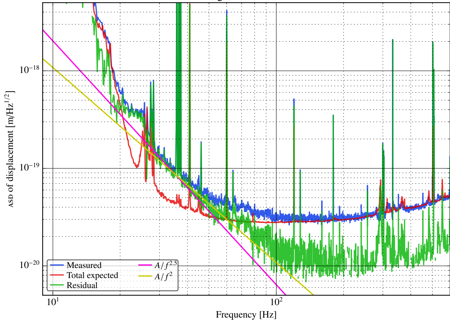
aLIGO H1 freerunning DARM, 2015-10-24 13:30:00 Z
