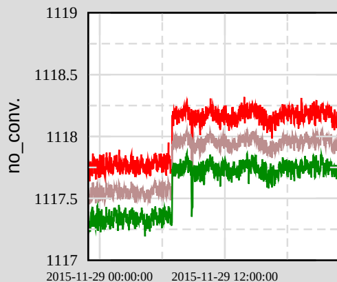
Ch 1: H1:SUS-IM1_M1_DAMP_P_INMON
