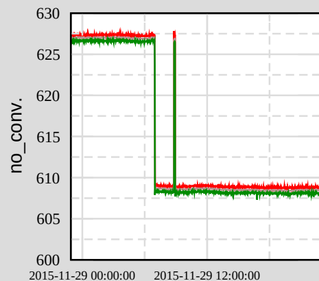
Ch 2: H1:SUS-IM1_M1_DAMP_Y_INMON
