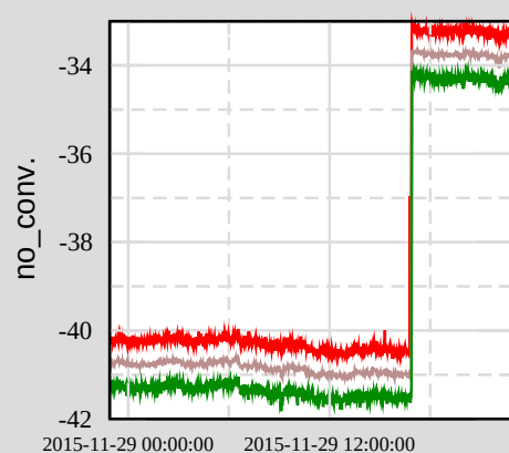
Ch 5: H1:SUS-IM3_M1_DAMP_P_INMON
