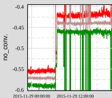
Ch 8: H1:SUS-IM4_M1_DAMP_Y_INMON
