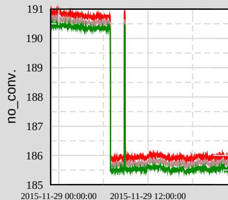
Ch 1: H1:SUS-IM1_M1_DAMP_P_INMON
