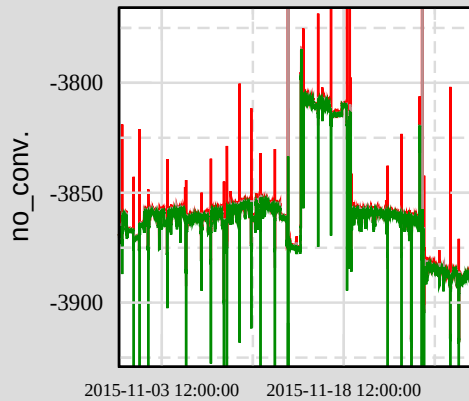
Ch 7: H1:SUS-IM4_M1_DAMP_P_INMON
