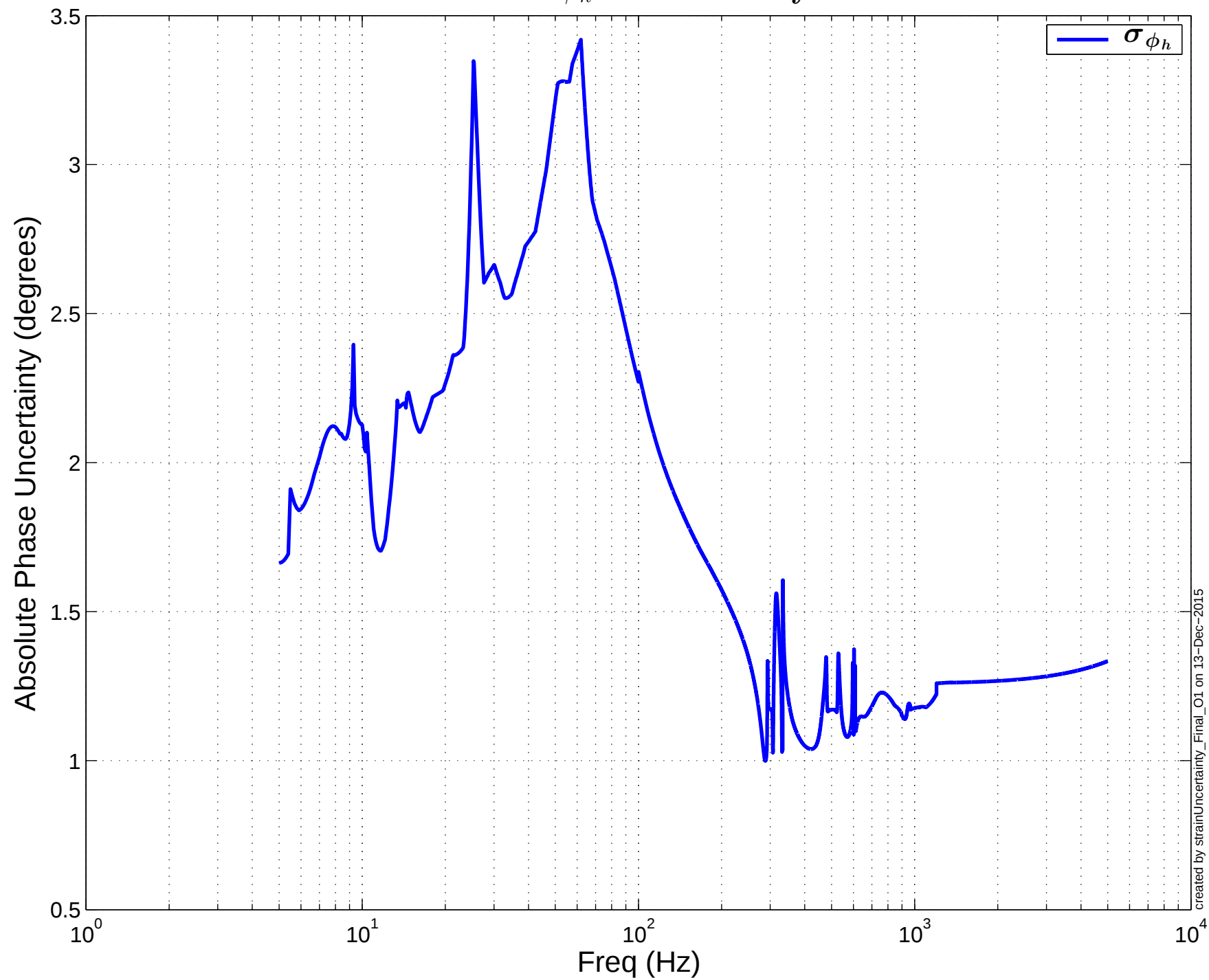
LHO C01 \phi_h Uncertainty Nominal
