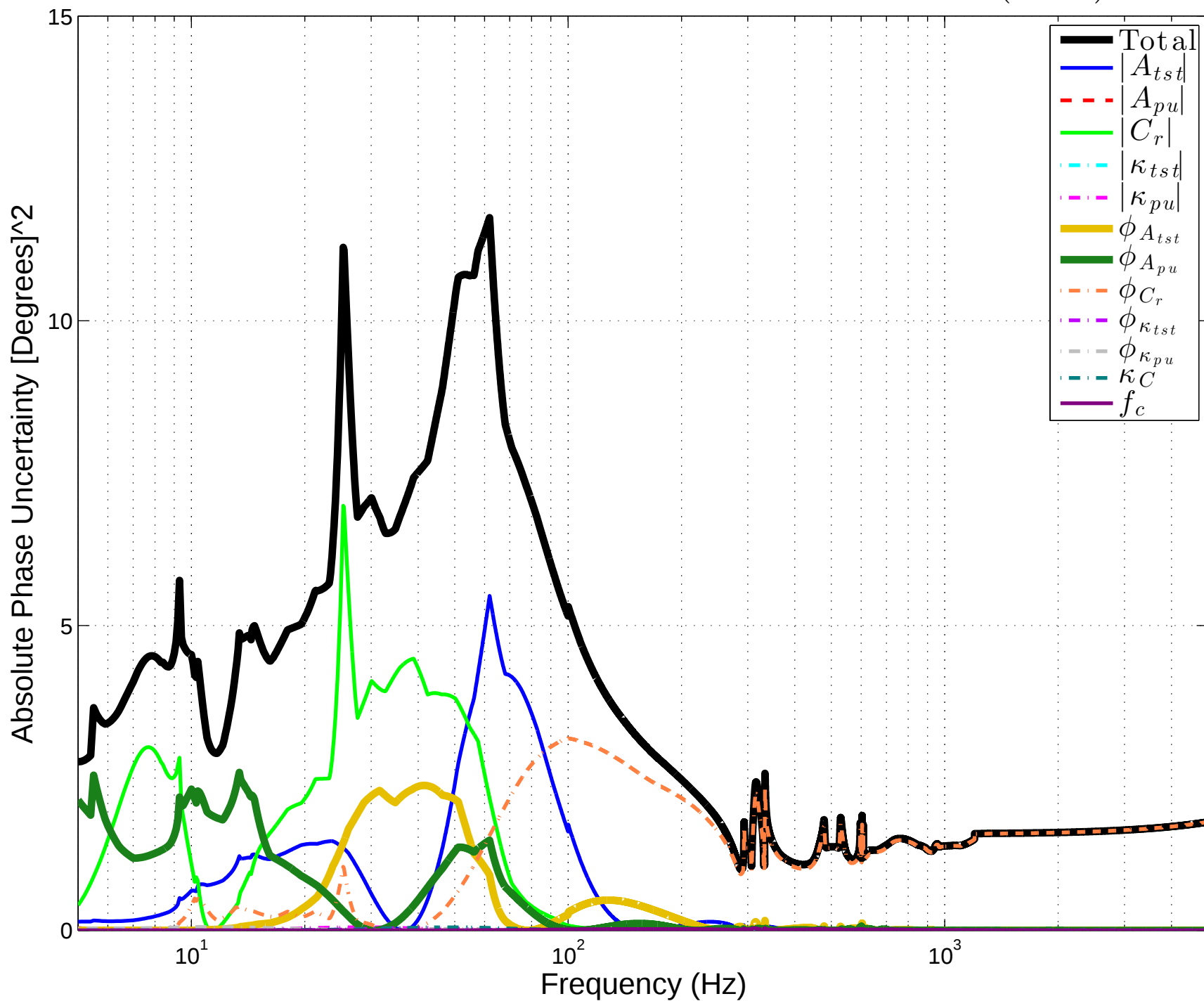
LHO C01 Squared Phase Uncertainty Components Nominal \left(\frac{\partial \phi_h}{\partial (legend)}\right)^2 \sigma_{(legend)}^2
