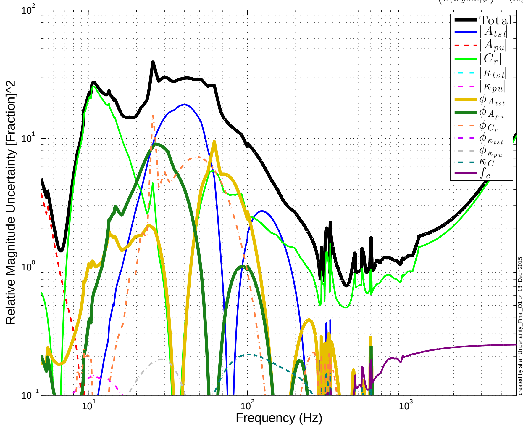
LHO C01 Squared Magnitude Uncertainty Components Nominal \left(\frac{\partial|h|}{\partial(\text{legend})}\frac{1}{|h|}\right)^2 \sigma_{(\text{legend})}^2
