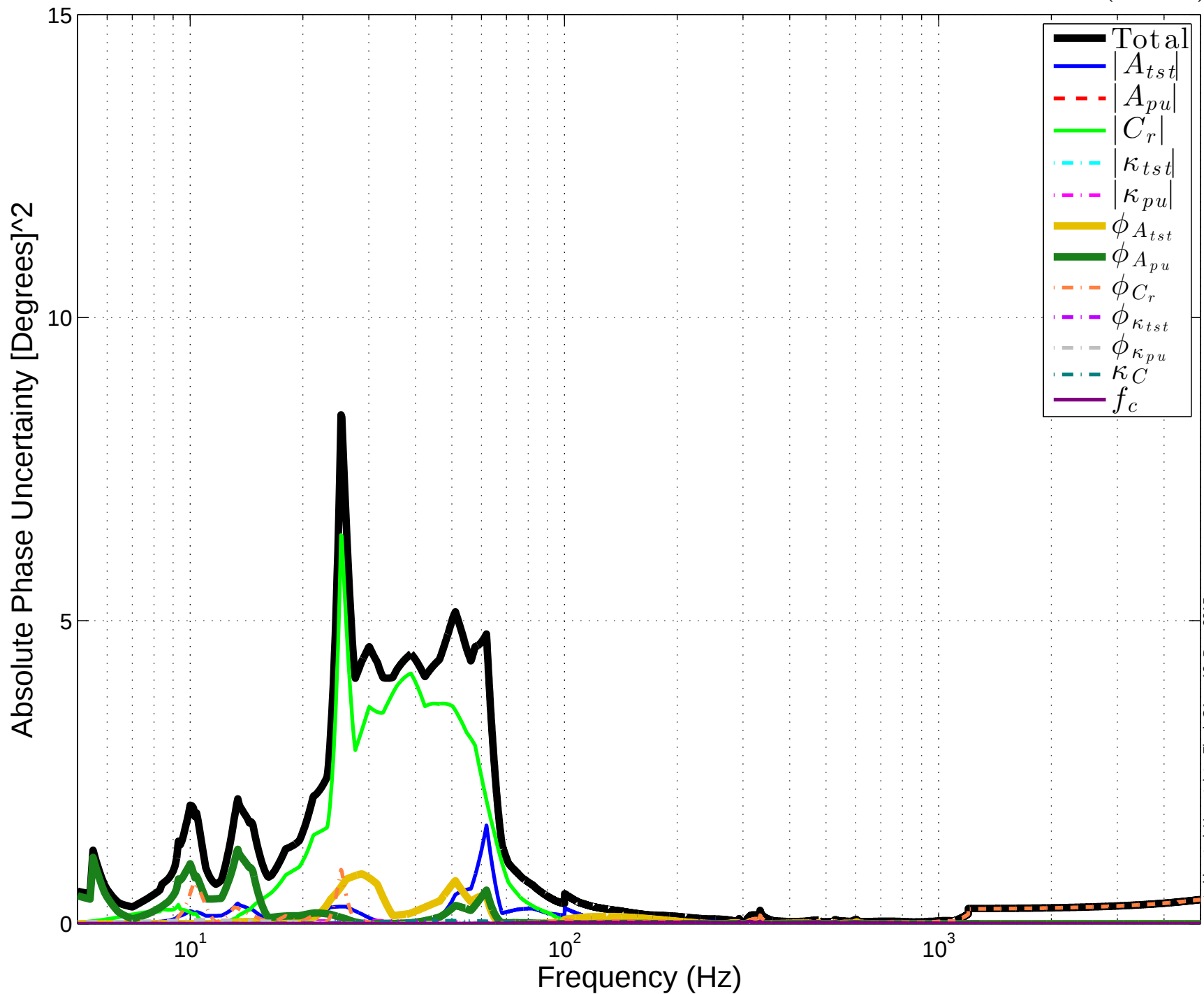
LHO C01 Squared Phase Uncertainty Components Systematic Corrected \left(\frac{\partial \phi_h}{\partial (legend)}\right)^2 \sigma_{(legend)}^2
