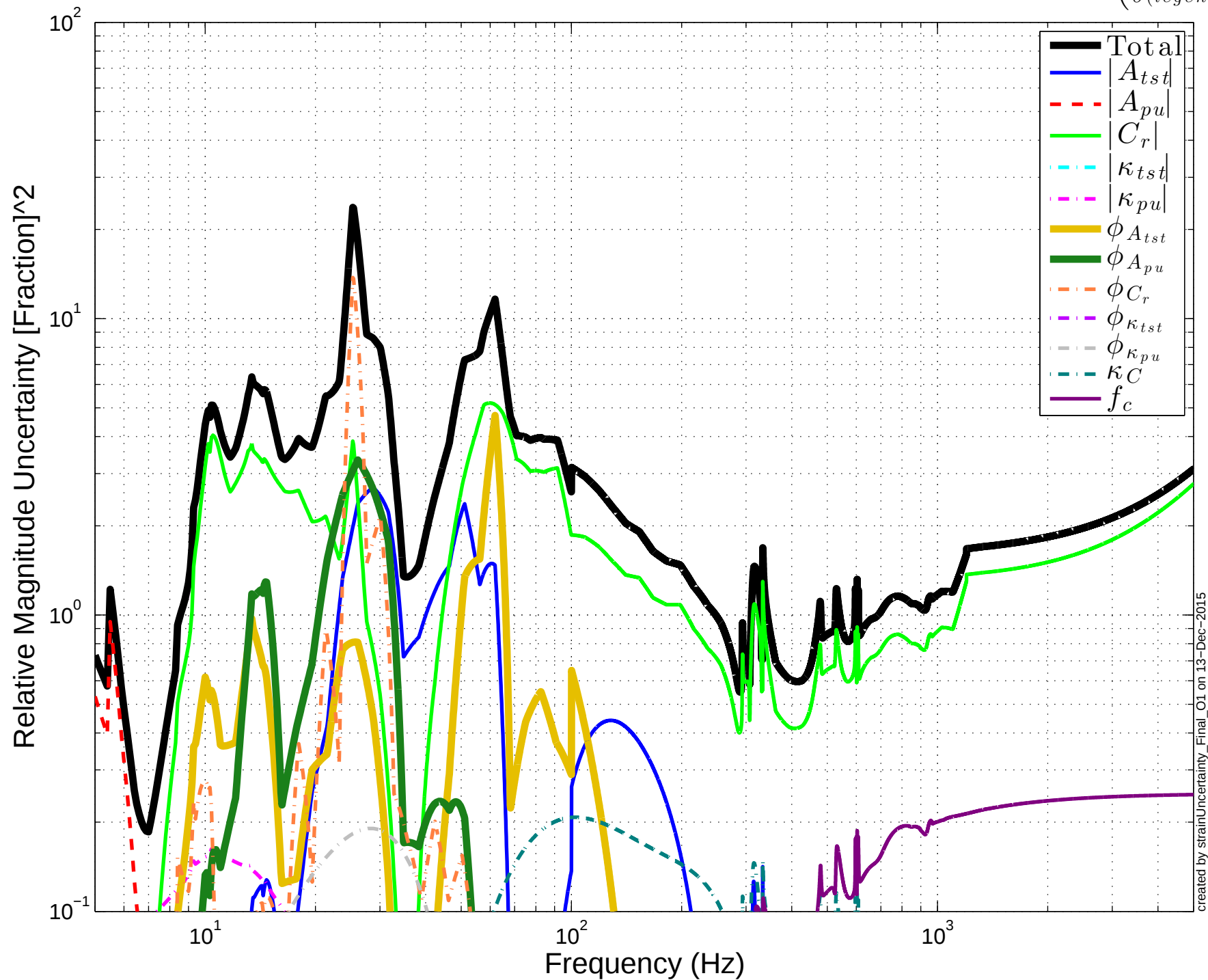
LHO C01 Squared Magnitude Uncertainty Components Systematic Corrected \left(\frac{\partial|h|}{\partial(\text{legend})}\frac{1}{d|h|}\right)^2 \sigma_{(leg\epsilon}^2
