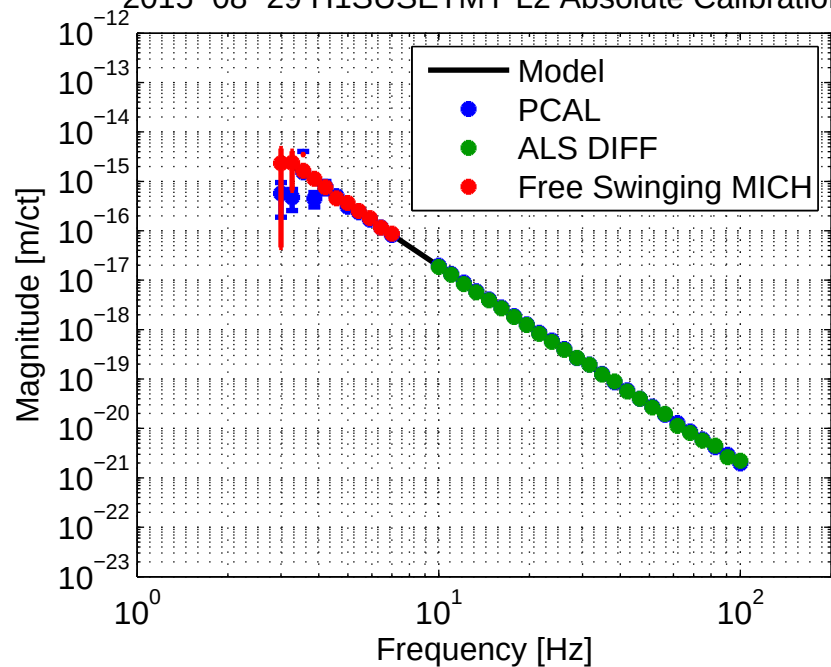
2015-08-29 H1SUSEMY L2 Absolute Calibration
