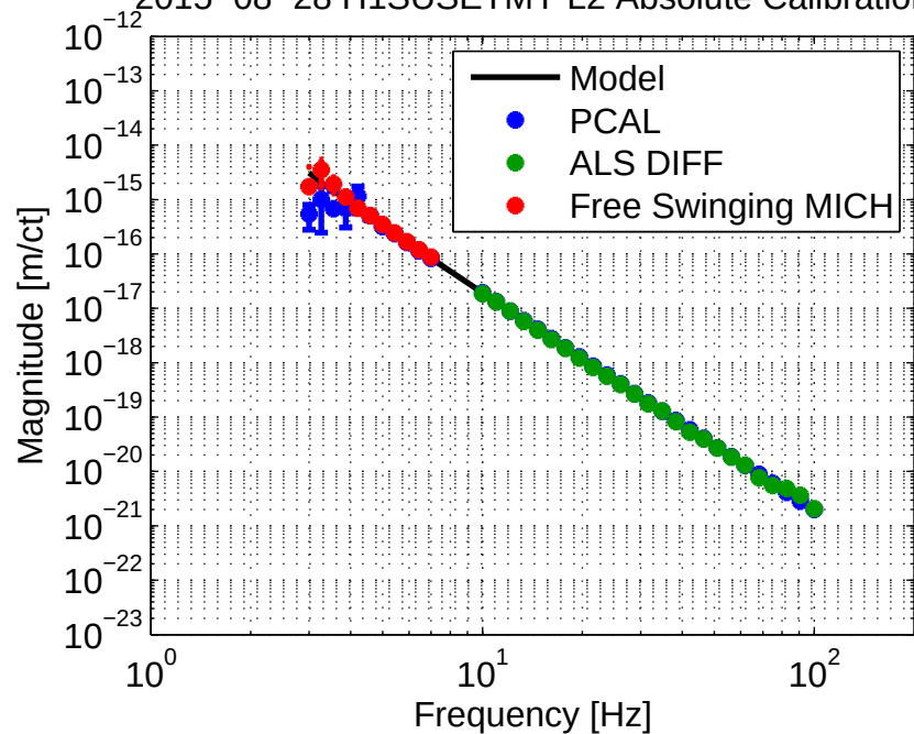
2015-08-28 H1SUSEMY L2 Absolute Calibration
