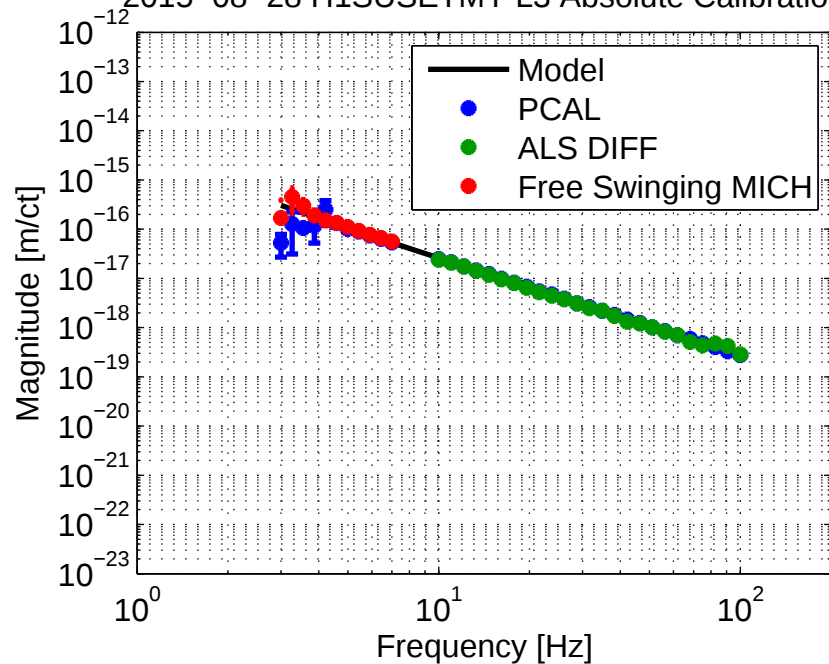
2015-08-28 H1SUSEMY L3 Absolute Calibration
