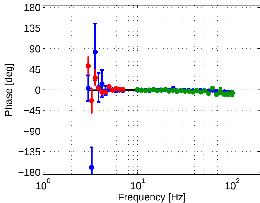
Fit Actuation Strength: 1.55\text{e-}10 \text{ [N/V}_{\text{ESD}}^2]
