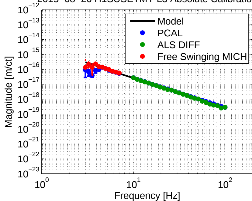
2015-08-26 H1SUSEMY L3 Absolute Calibration
