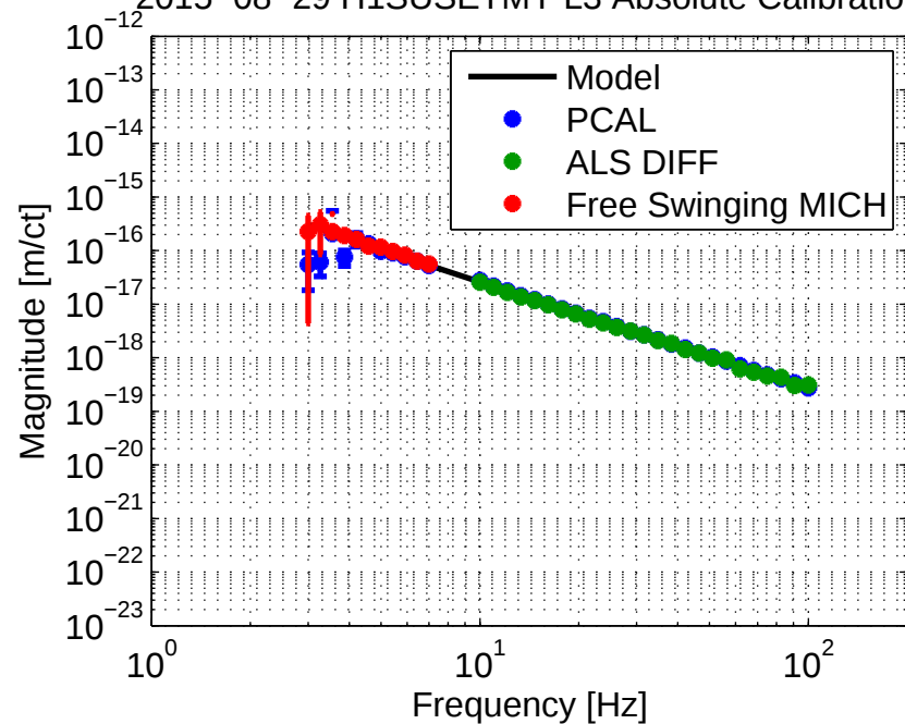
2015-08-29 H1SUSEMY L3 Absolute Calibration
