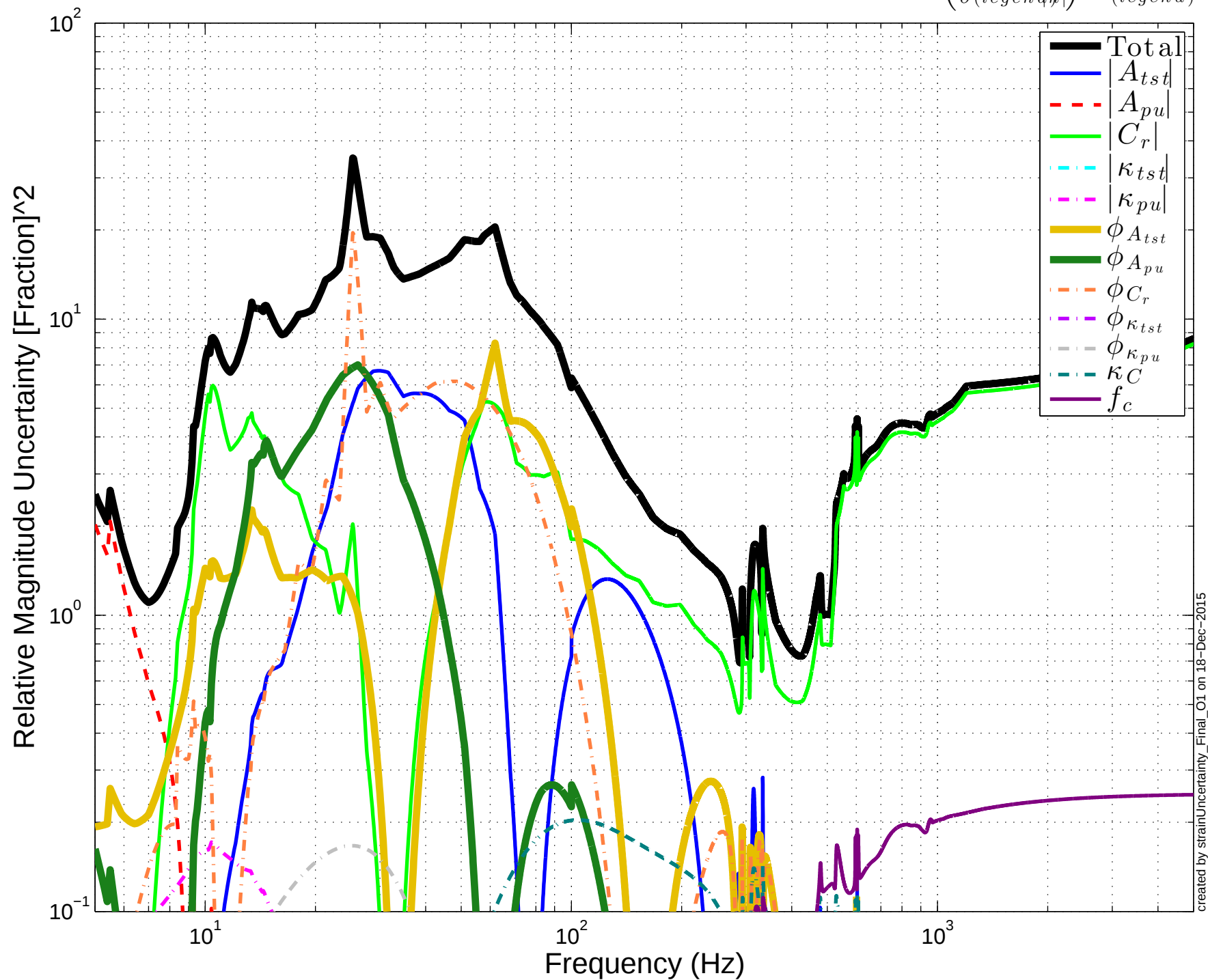
LHO C02 Squared Magnitude Uncertainty Components \left(\frac{\partial|h|}{\partial(\text{legend})}\frac{1}{h}\right)^2 \sigma_{(\text{legend})}^2
