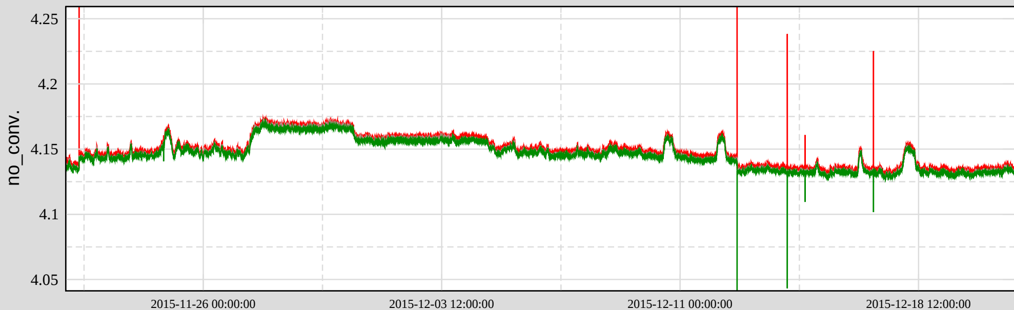
Ch 1: H1:LSC-MOD_RF45_AM_CTRL_OUT_DQ
