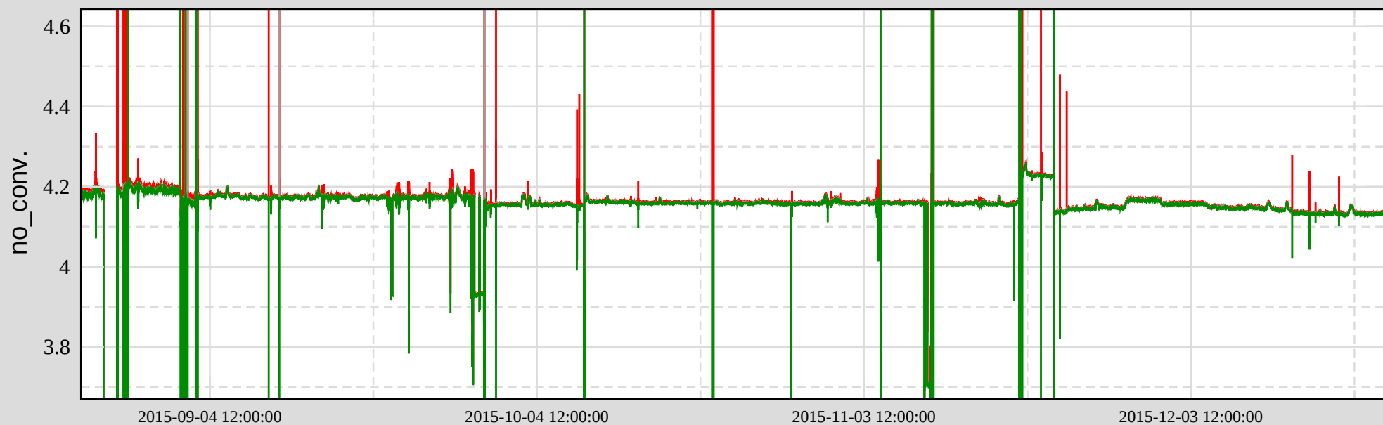
Ch 1: H1:LSC-MOD_RF45_AM_CTRL_OUT_DQ
