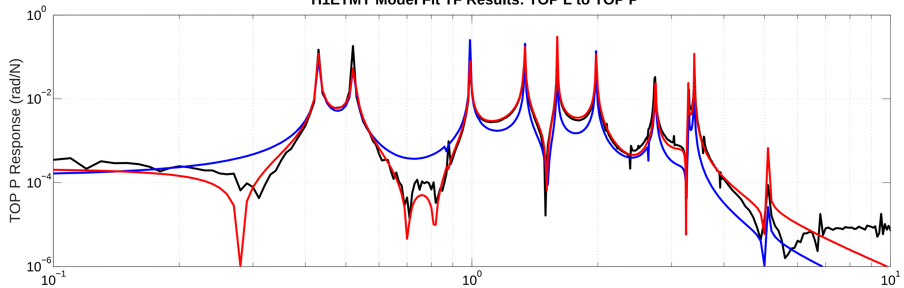
H1ETMY Model Fit TF Results: TOP L to TOP P
