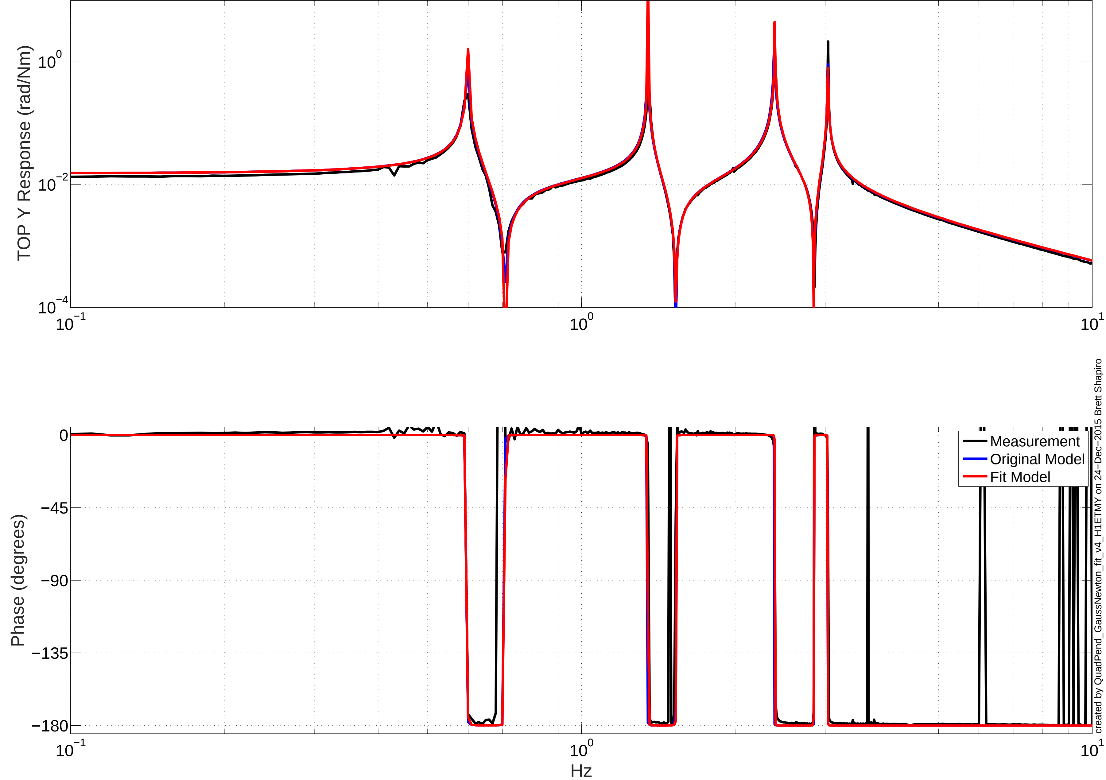
H1ETMY Model Fit TF Results: TOP Y to TOP Y
