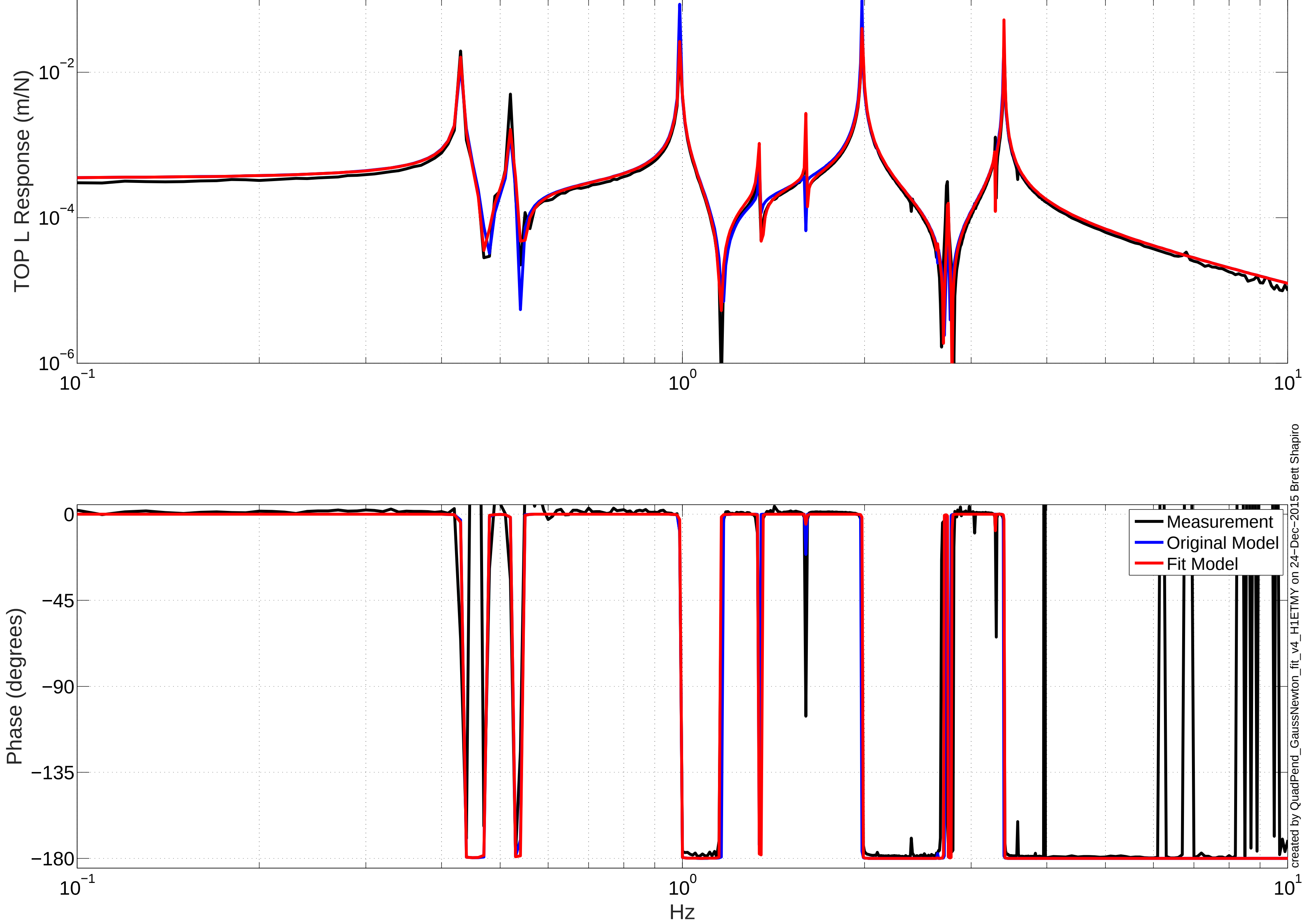
H1ETMY Model Fit TF Results: TOP L to TOP L
