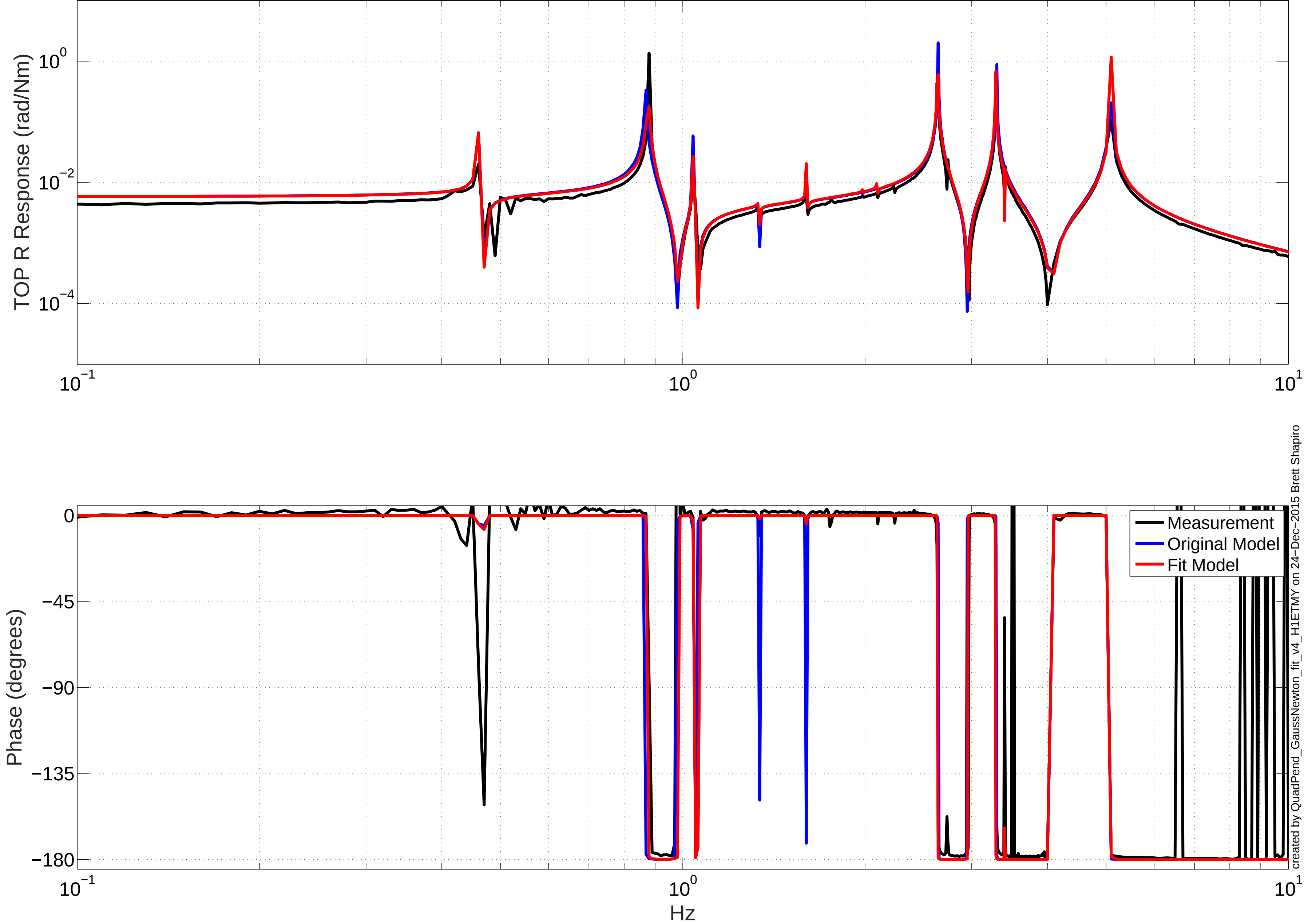
H1ETMY Model Fit TF Results: TOP R to TOP R
