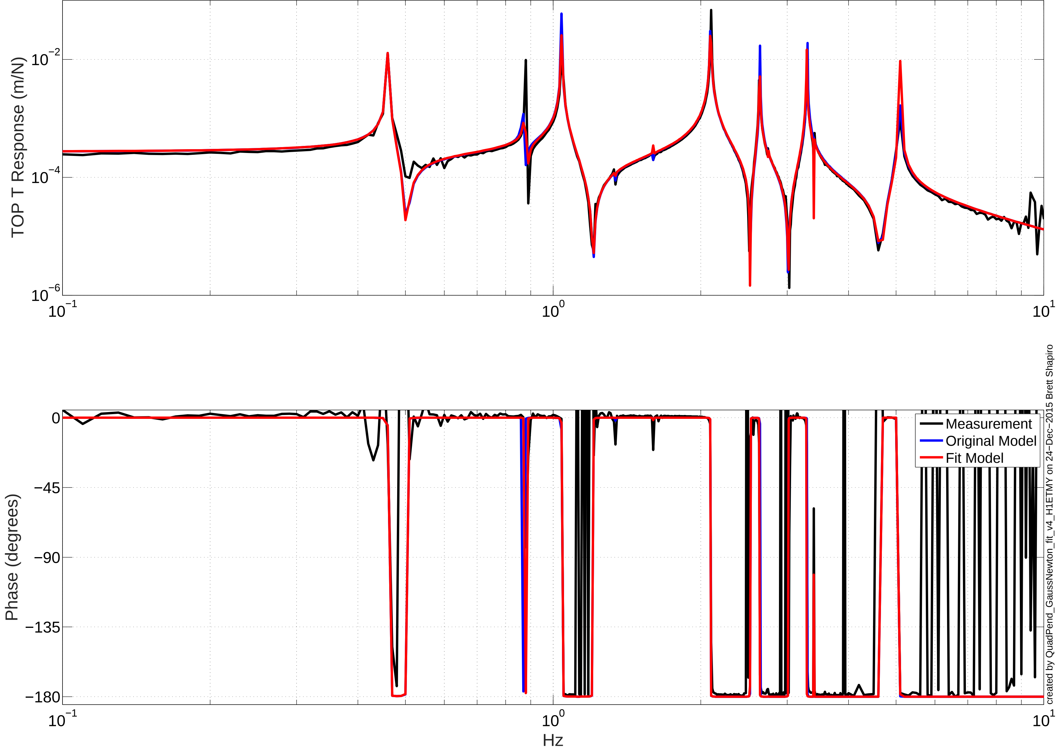
H1ETMY Model Fit TF Results: TOP T to TOP T
