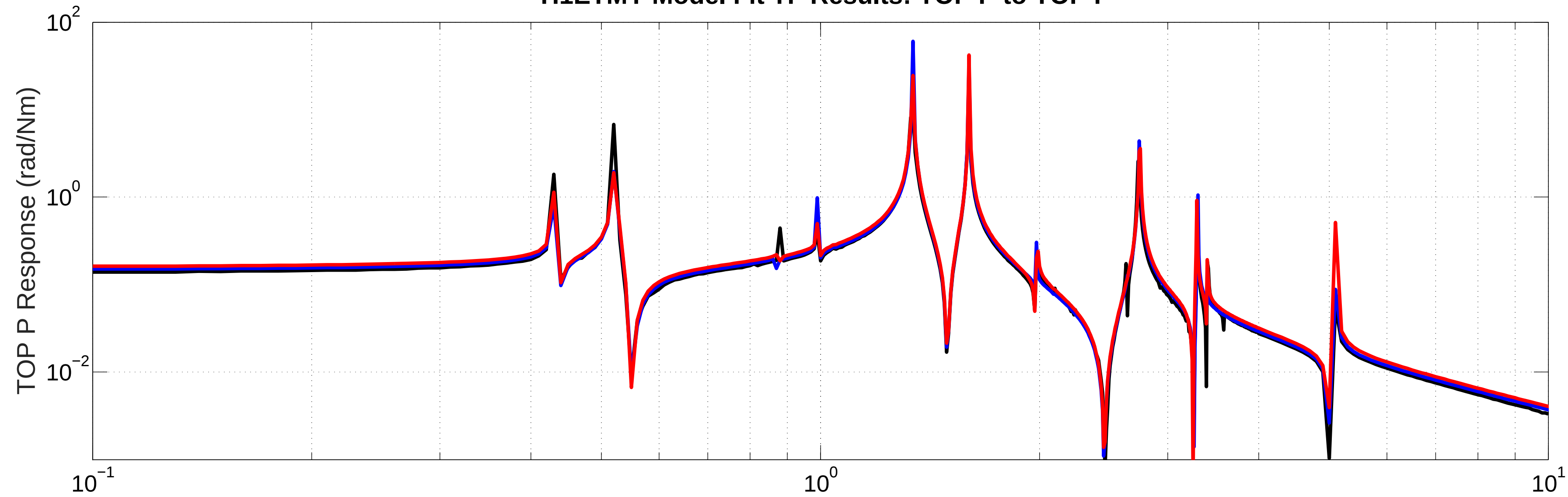
H1ETMY Model Fit TF Results: TOP P to TOP P
