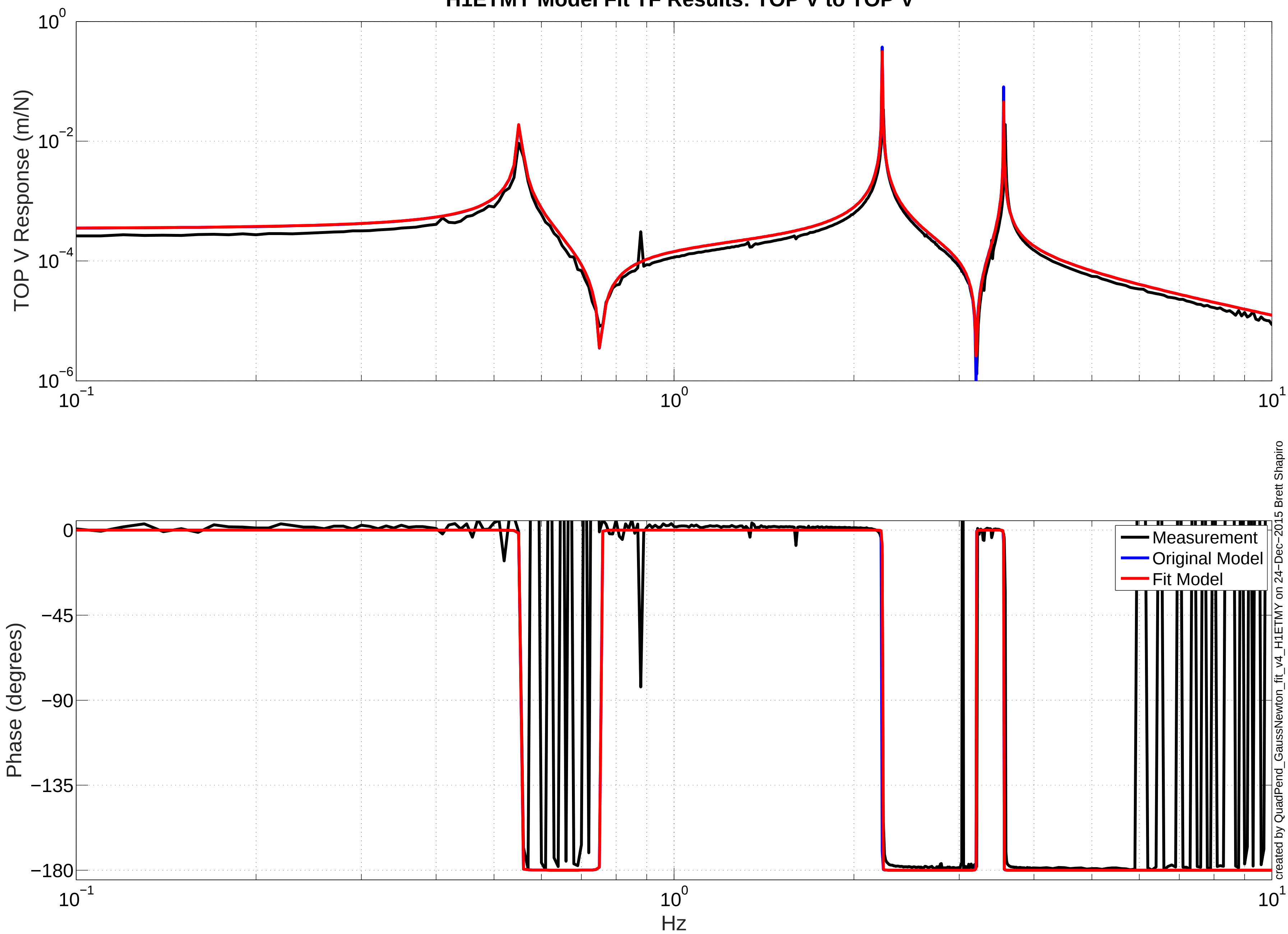
H1ETMY Model Fit TF Results: TOP V to TOP V
