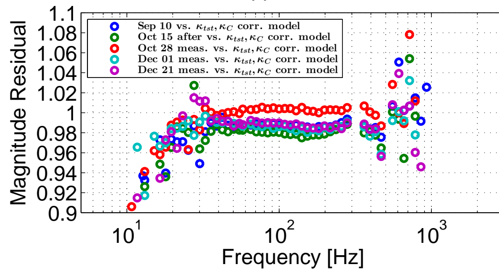
H1 DARM Open Loop Gain TF Comparison Meas. / KappaCorrectedModel
