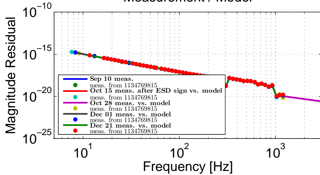
H1 Actuation Comparison Measurement / Model
