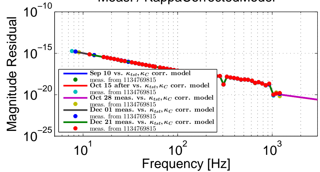
H1 Actuation Comparison Meas. / KappaCorrectedModel
