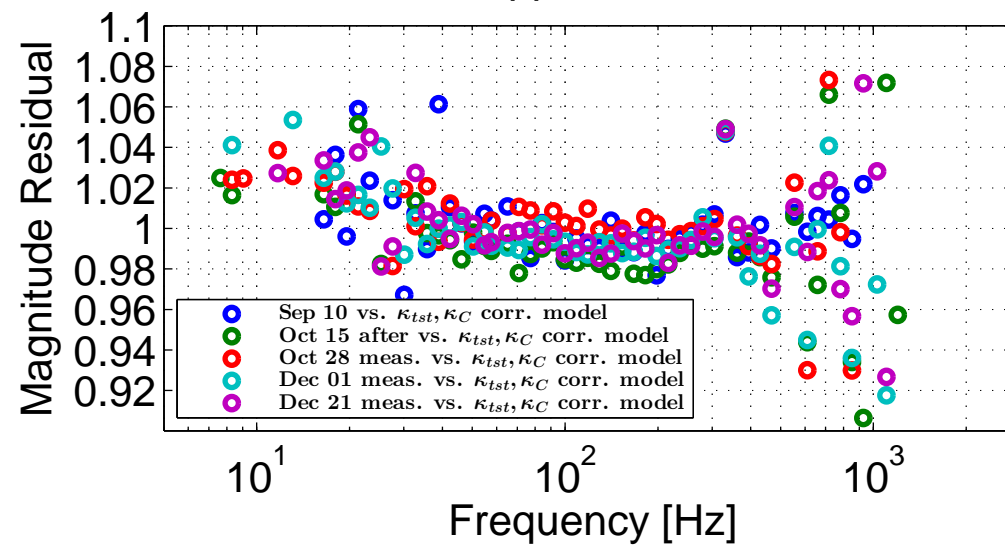
H1 Actuation Residual Meas. / KappaCorrectedModel
