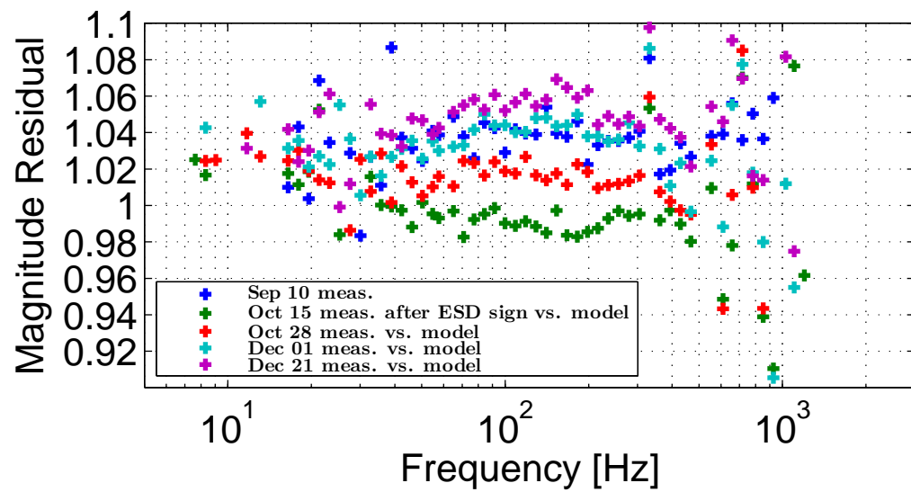
H1 Actuation Residual Measurement / Model
