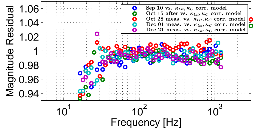
H1 Sensing Residual Meas. / KappaCorrectedModel
