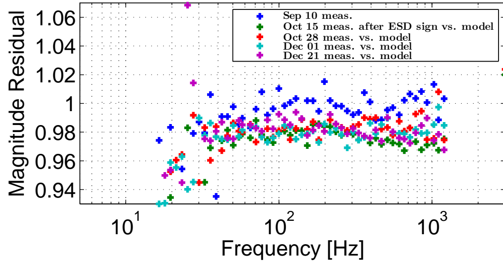
H1 Sensing Residual Measurement / Model
