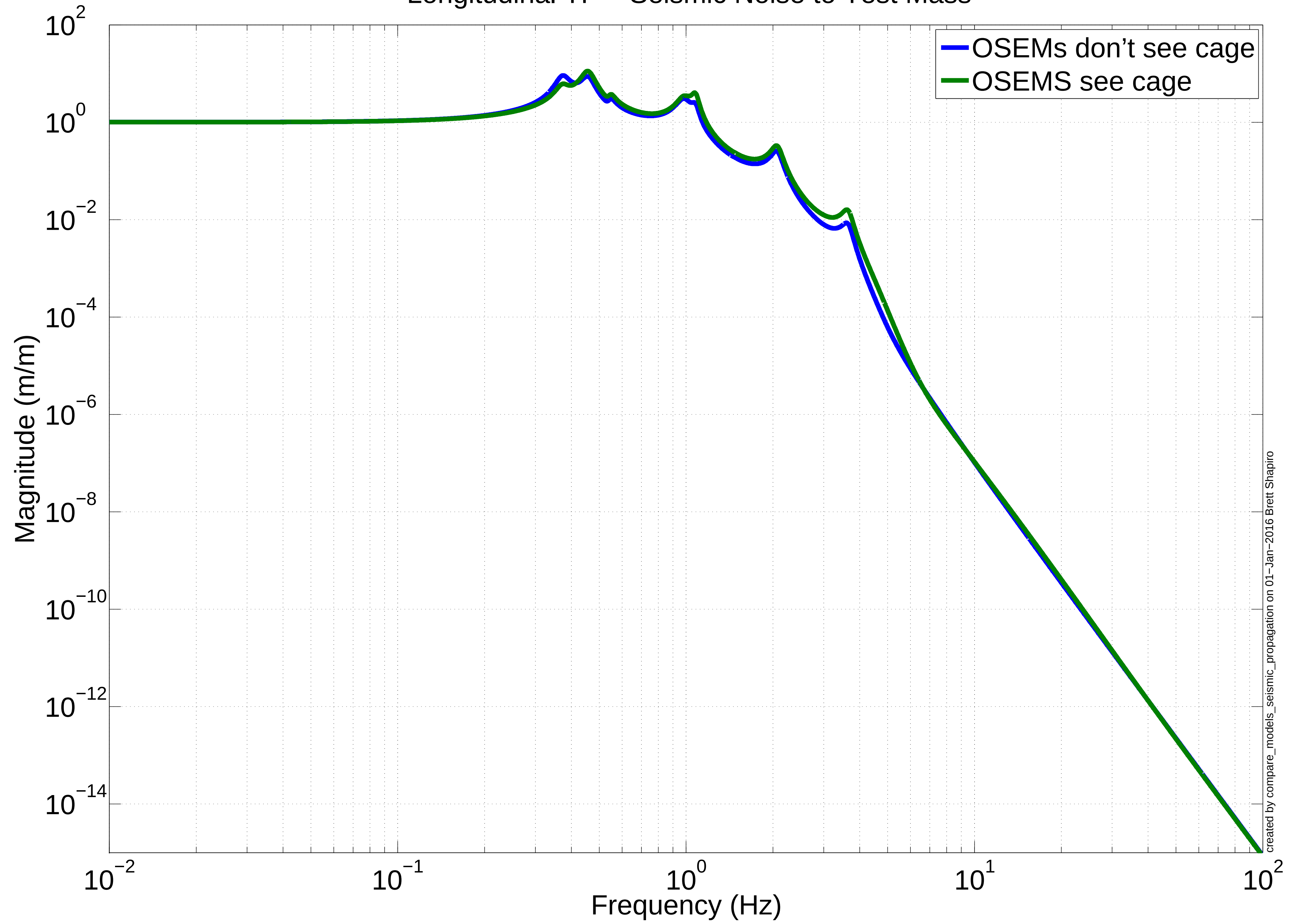
Longitudinal TF – Seismic Noise to Test Mass
