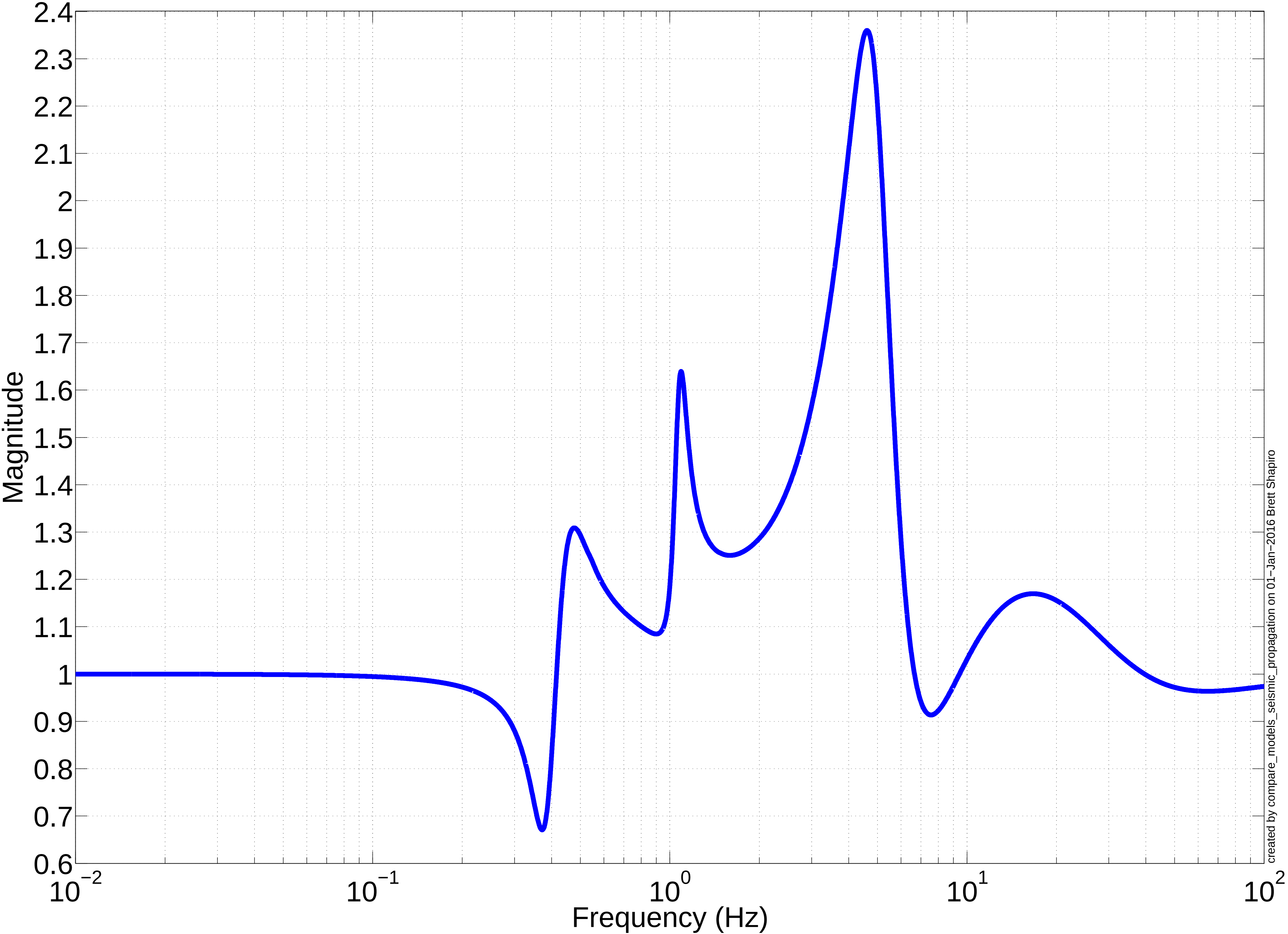
Longitudinal Seismic to Test Mass TF Ratio – (OSEMS see cage) / (OSEMs don't see cage)
