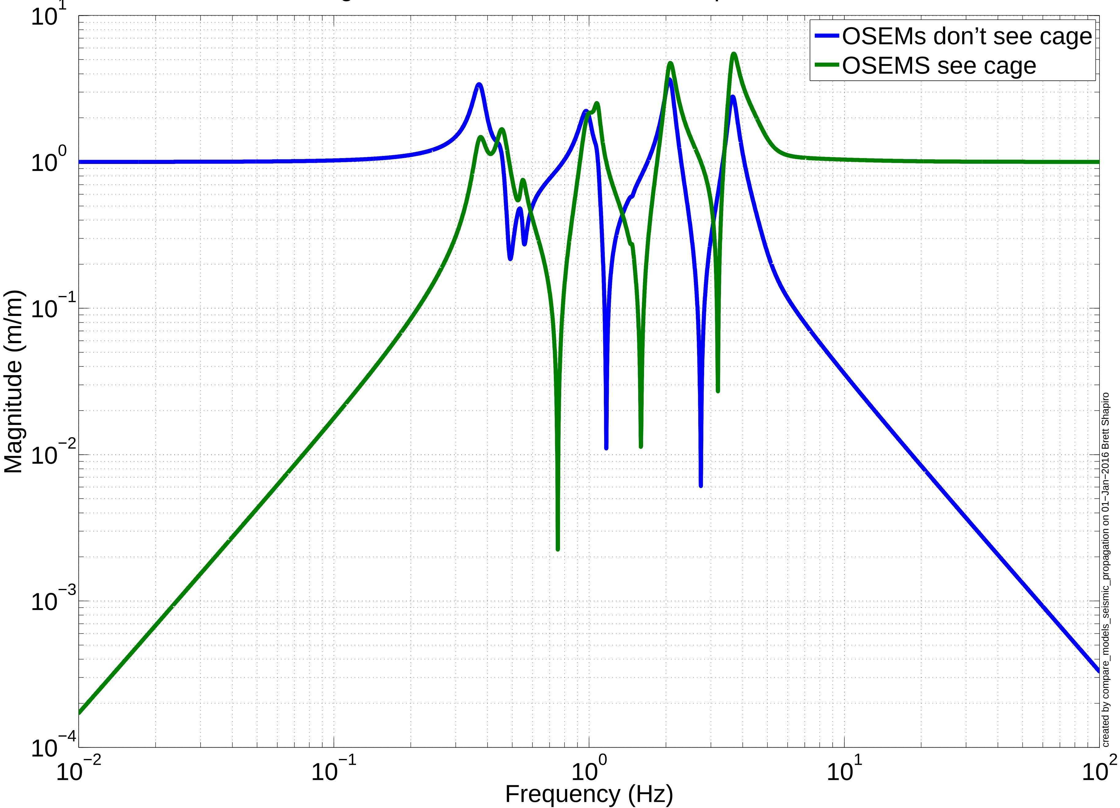
Longitudinal TF – Seismic Noise to Top Mass OSEMs
