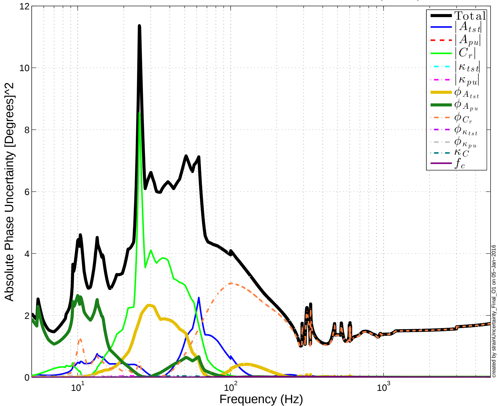
LHO C02 Squared Phase Uncertainty Components \left(\frac{\partial \phi_h}{\partial (legend)}\right)^2 \sigma_{(legend)}^2
