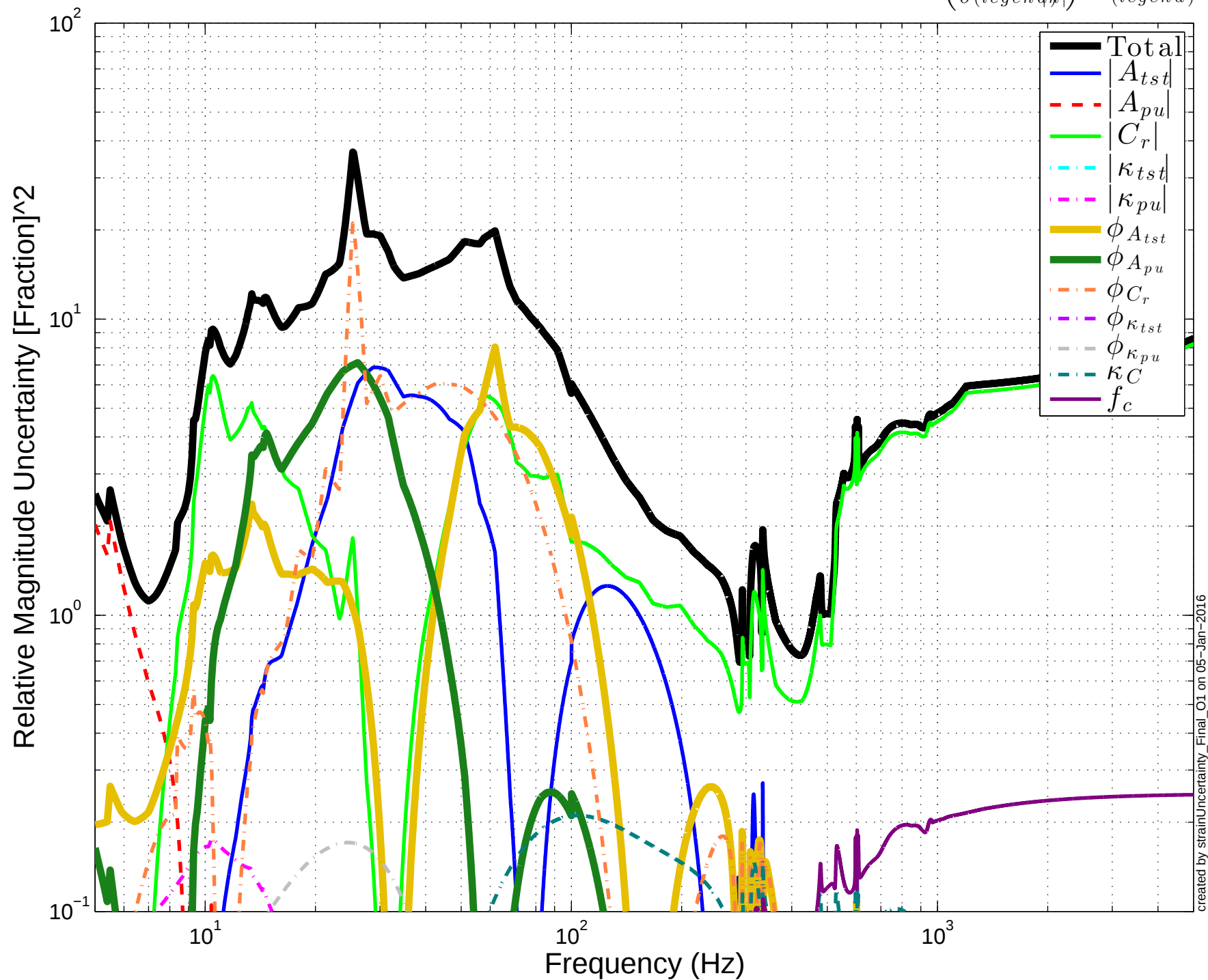
LHO C02 Squared Magnitude Uncertainty Components \left(\frac{\partial|h|}{\partial(\text{legend})}\frac{1}{h}\right)^2\sigma_{(\text{legend})}^2
