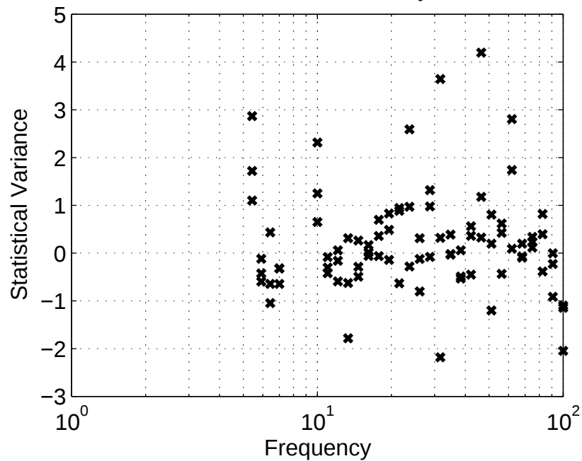
Phase Stat Var = Res - Syst Fit
