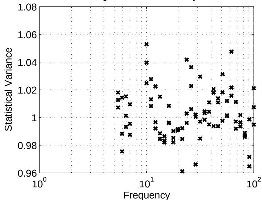
L1 Mag Stat Var = Res - Syst Fit
